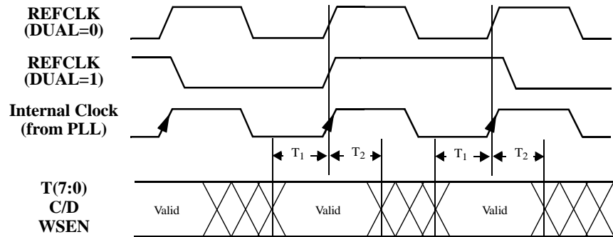
Figure 14: Transmit Input Timing Waveforms with TMODE = 10X
