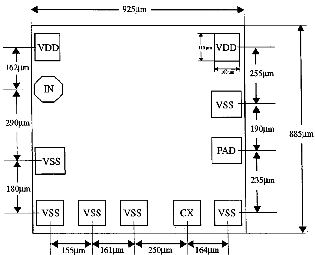
Figure 1: VSC7902 Bonding Pad Diagram
