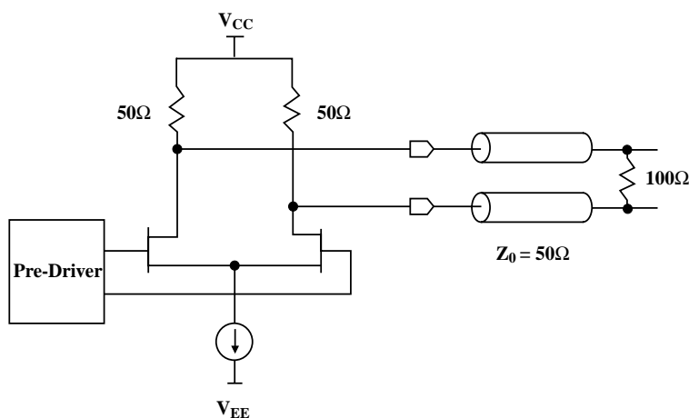
Figure 13: High-Speed Output Termination
