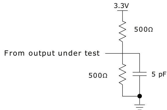
FIGURE 3-10: TEST CIRCUIT FOR TDO DISABLE TIME
