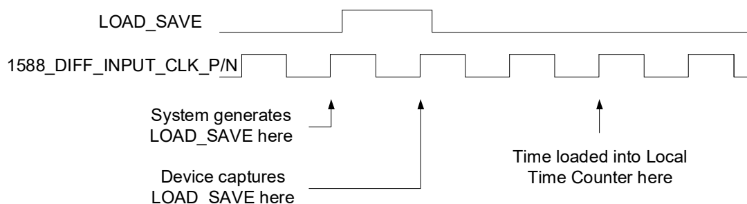
FIGURE 1-22: LOCAL TIME COUNTER LOAD/SAVE TIMING
