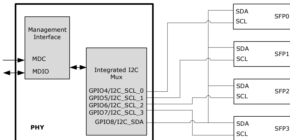
FIGURE 1-27: TWO-WIRE SERIAL MUX WITH SFP CONTROL AND STATUS
