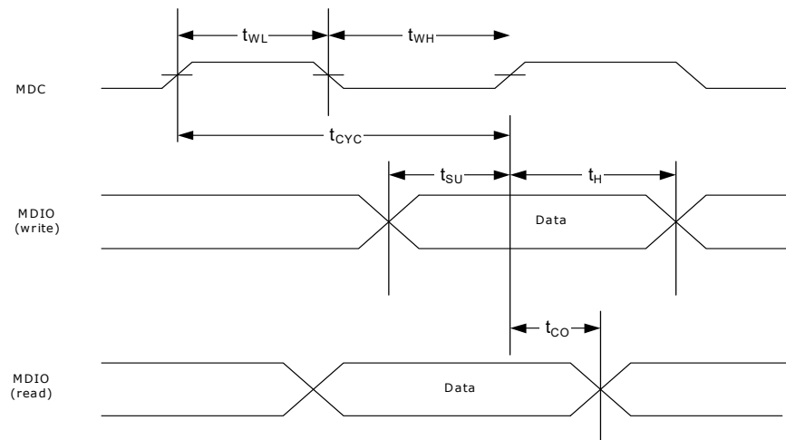
FIGURE 3-11: SERIAL MANAGEMENT INTERFACE TIMING
