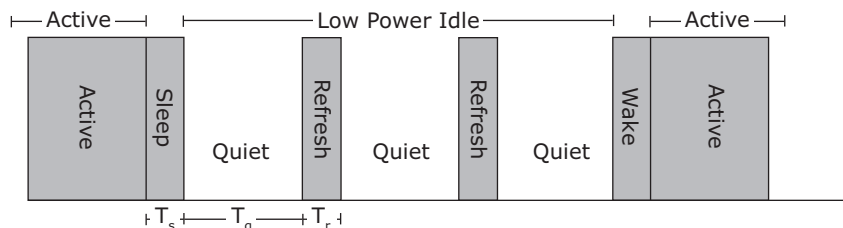
FIGURE 1-14: LOW POWER IDLE OPERATION
