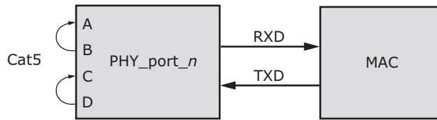
FIGURE 1-31: CONNECTOR LOOPBACK DIAGRAM
