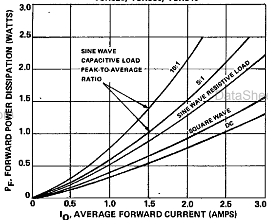
FORWARD POWER DISSIPATION VSK320, VSK330, VSK340
