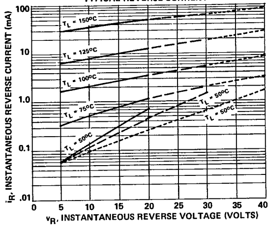
TYPICAL REVERSE CURRENT
