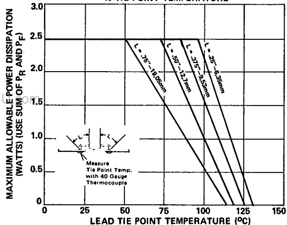
MAXIMUM ALLOWABLE POWER DISSIPATION vs TIE POINT TEMPERATURE
