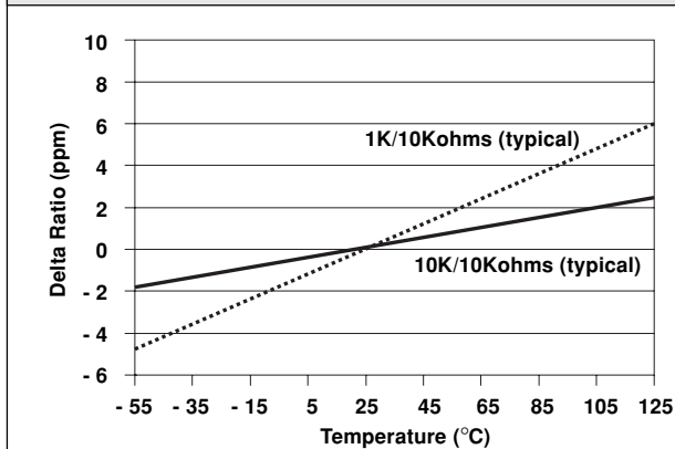
FIGURE 2 - DELTA RATIO VERSUS TEMPERATURE
