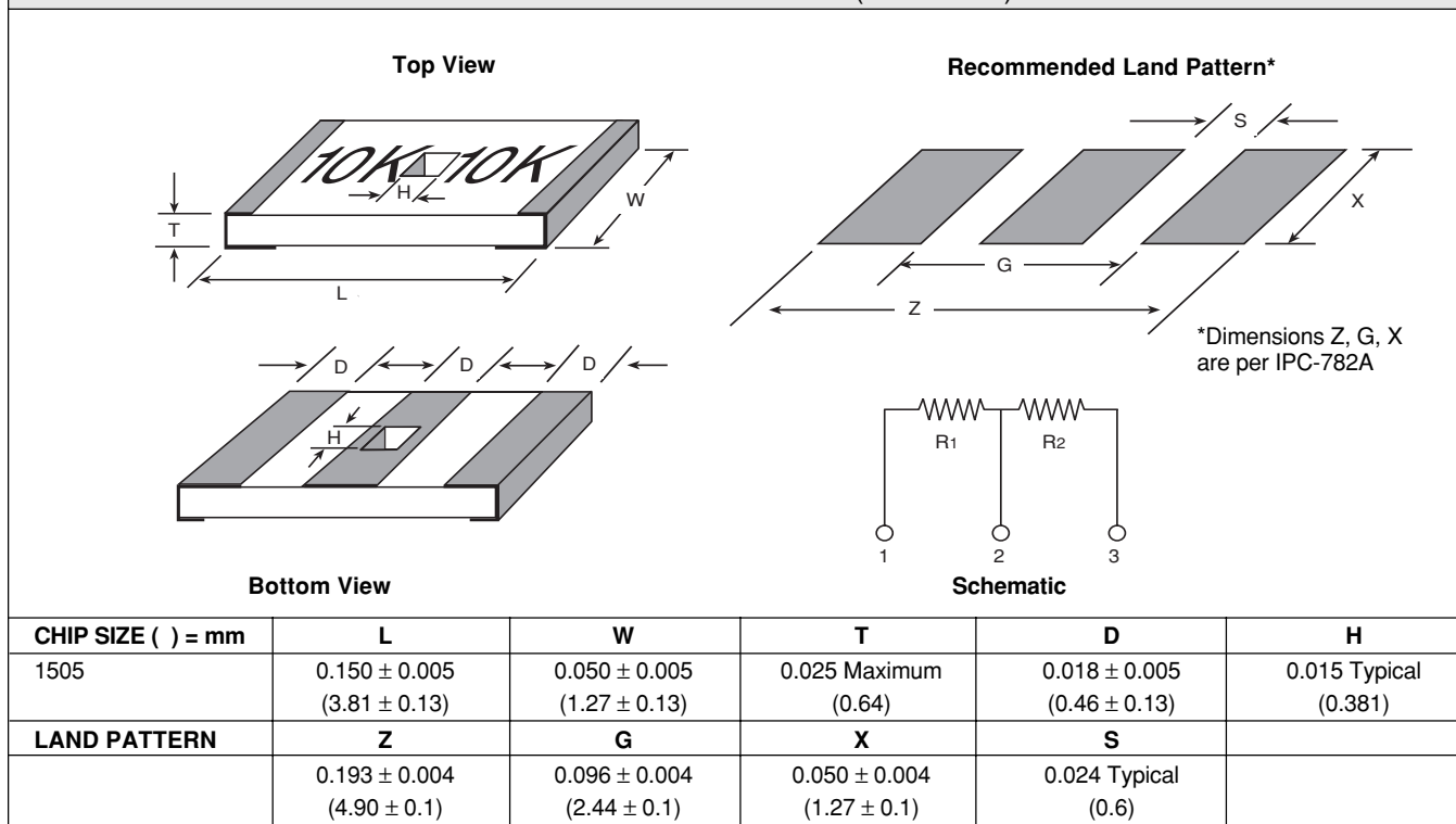
FIGURE 3 - MODEL VSM1505D DIMENSIONS in inches (millimeters)
