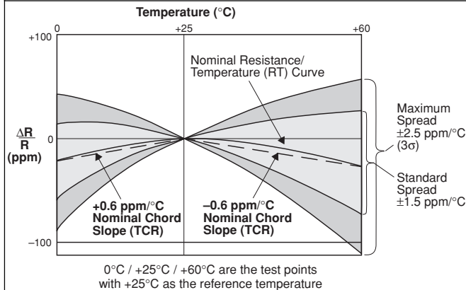
FIGURE 2 - DELTA RATIO VERSUS TEMPERATURE
