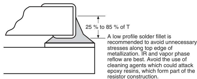
FIGURE 6 - RECOMMENDED MOUNTING
