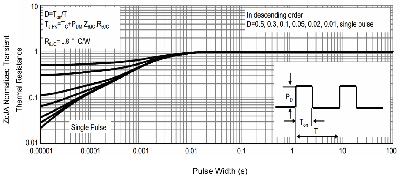
Fig9. Normalized Maximum Transient Thermal Impedance Tj -
