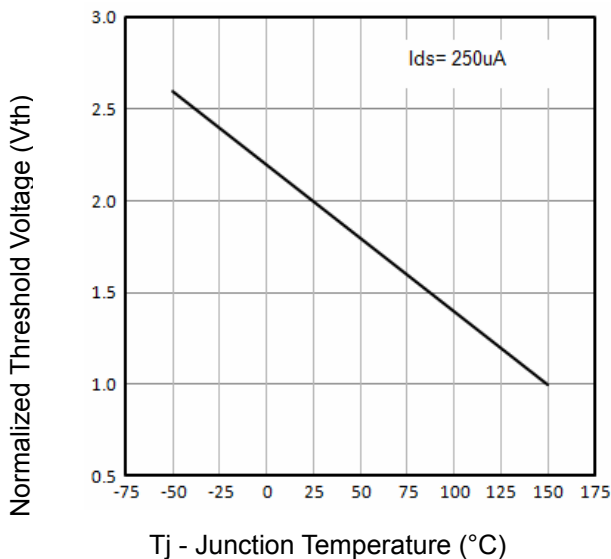
Fig5. Normalized Threshold Voltage Vs. Temperature
