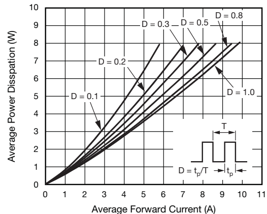
Fig. 2 - Forward Power Loss Characteristics Per Device
