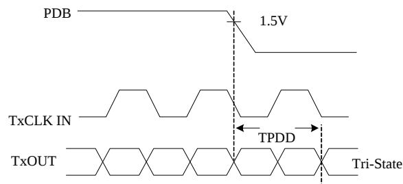
Figure 7. Tx Power Down Delay
