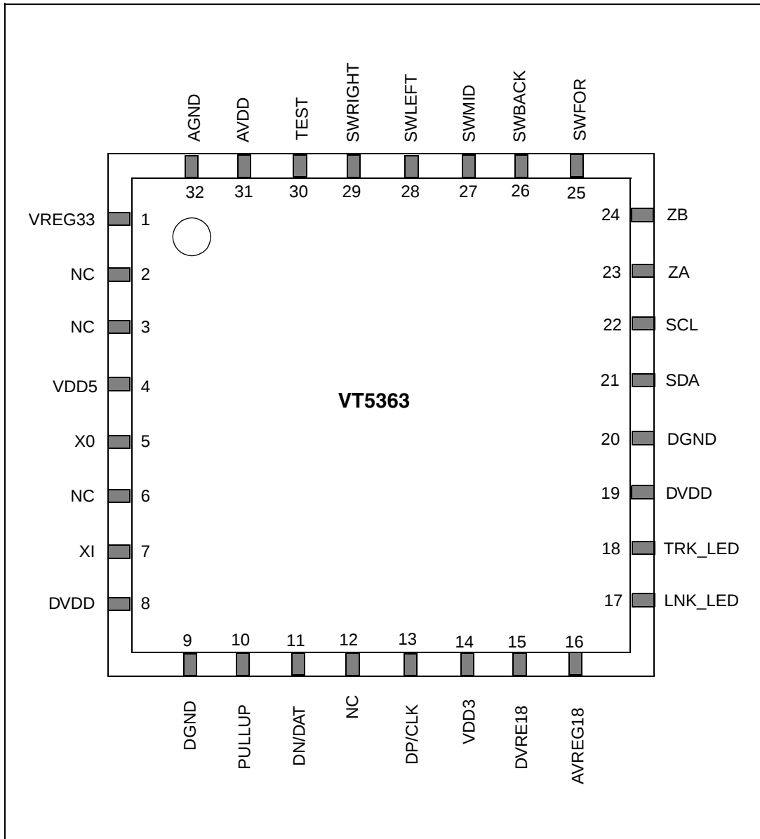
Figure 2. VT5363 pin assignment
