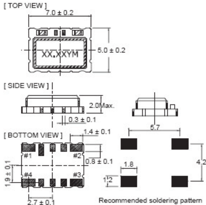
Contact Pads are gold over nickel Figure 3, Package drawing
