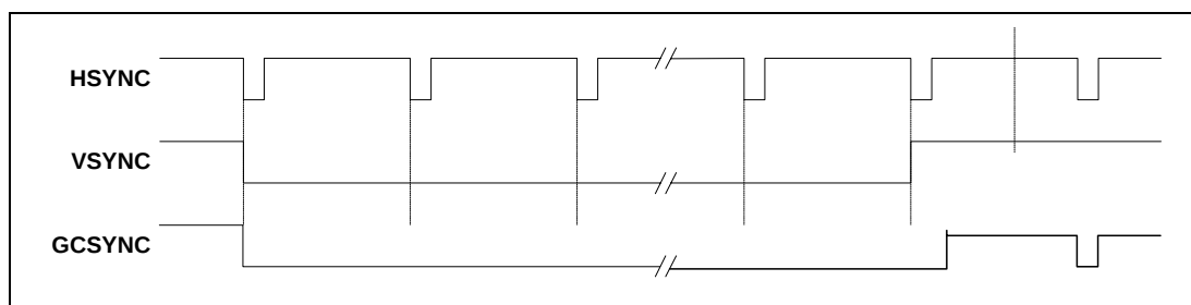
Figure 11.5.1 Video Output Synchronizations
