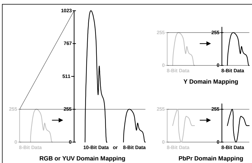
Figure 10.6.1.3 CLUT Mapping
