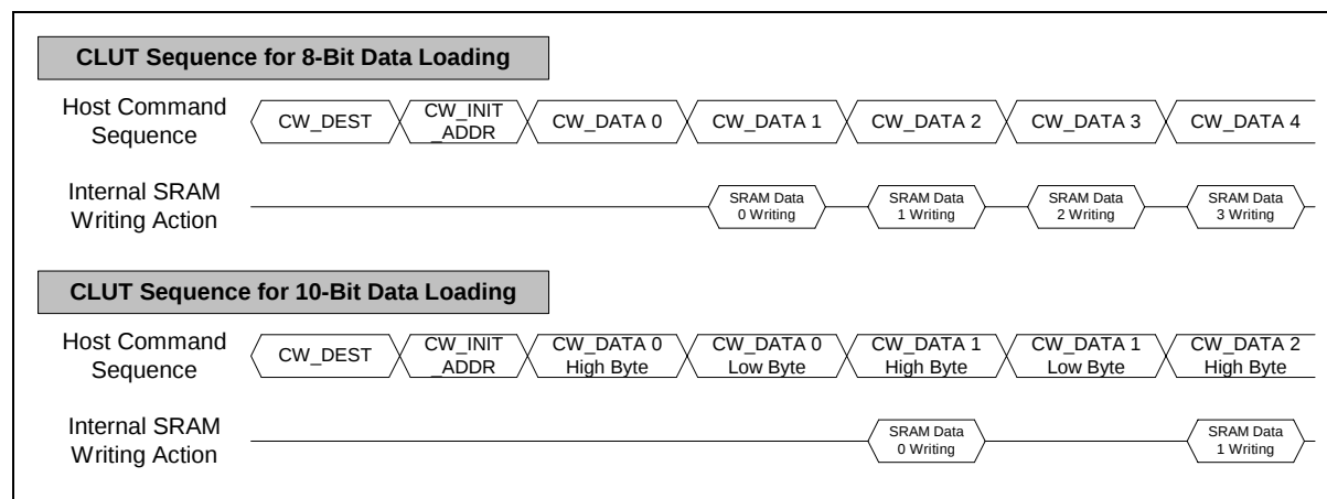
Figure 8.6.1.2 CLUT Programming Sequence Through Host Interface
