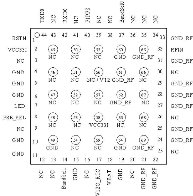
Figure-2a Venus838LPx Pin-Out Diagram
