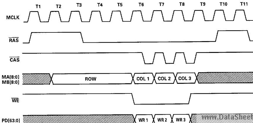
Figure 3-6. 1 Cycle EDO Write Timing
