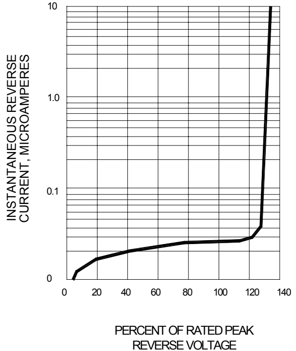
FIG. 4-TYPICAL REVERSE CHARACTERISTICS
