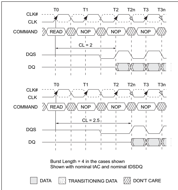
FIGURE 4 – CAS LATENCY
