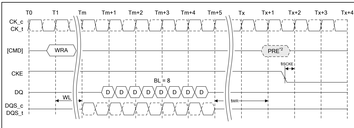
Figure 56 - Write with Auto Precharge to Power-Down Entry
