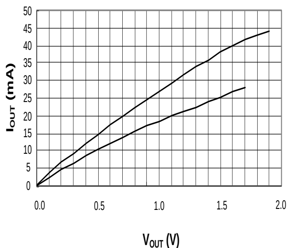
Pull-Down Characteristics
