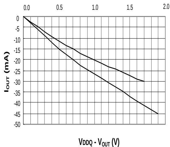
Pull-Up Characteristics
