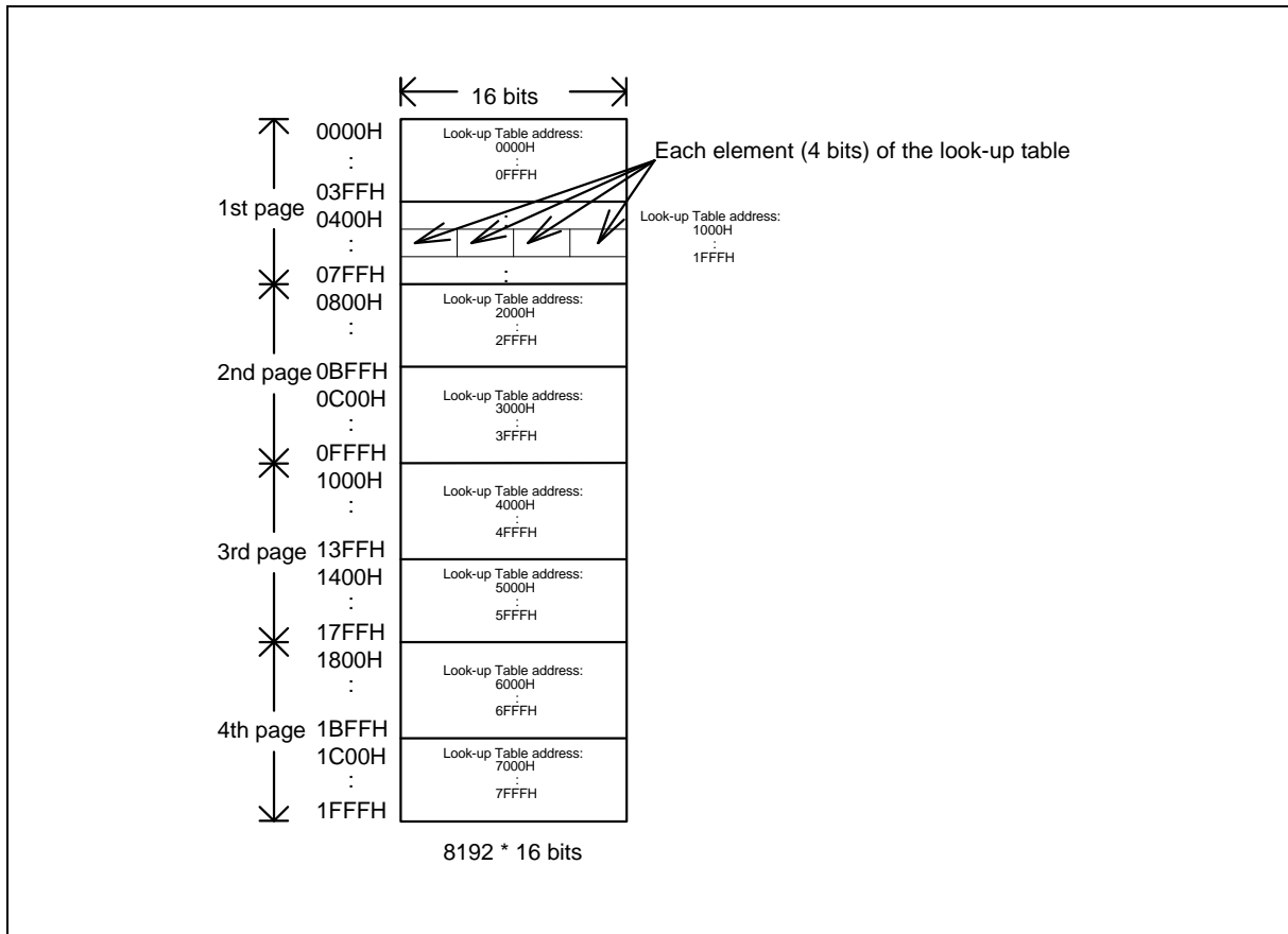
Figure 6-1 Program Memory Organization
