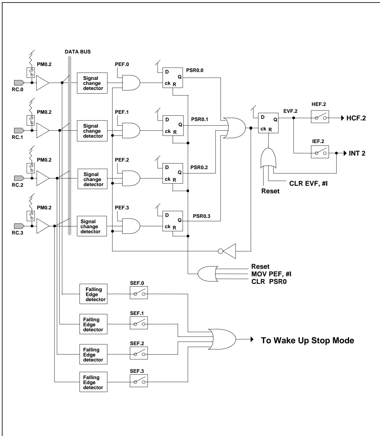
Figure 6-12 Architecture of Input Ports RC
