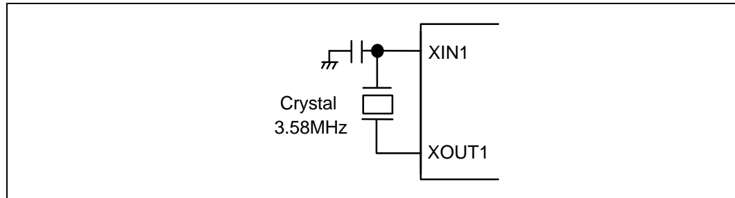
Figure 6-3 System clock oscillator Configuration
