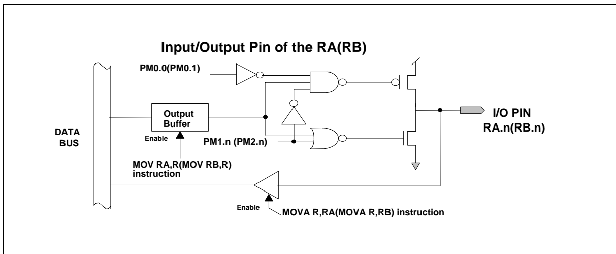
Figure 6-10 Architecture of RA (RB) Input/Output Pins
