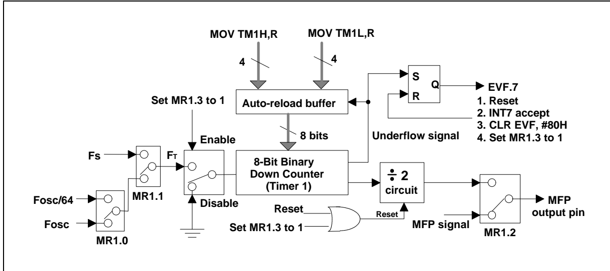
Figure 6-7 Organization of Timer 1
