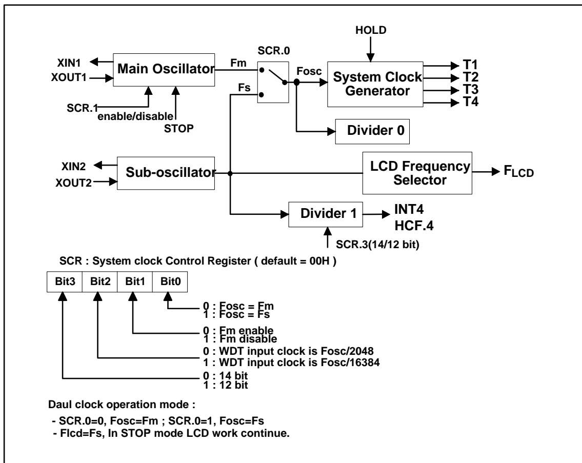
Figure 6-4 Organization of the dual-clock operation mode
