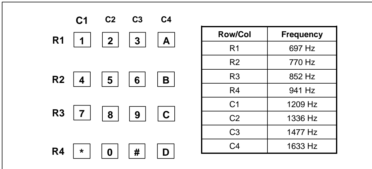
Figure 6-13 The relation between the touch tone keypad and the frequency
