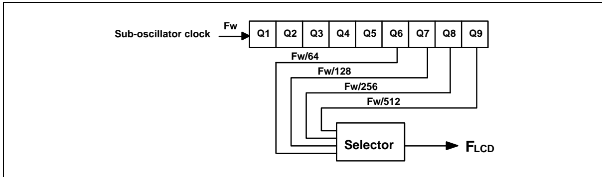
Figure 6-14 LCD alternating frequency (FLCD) circuit diagram
