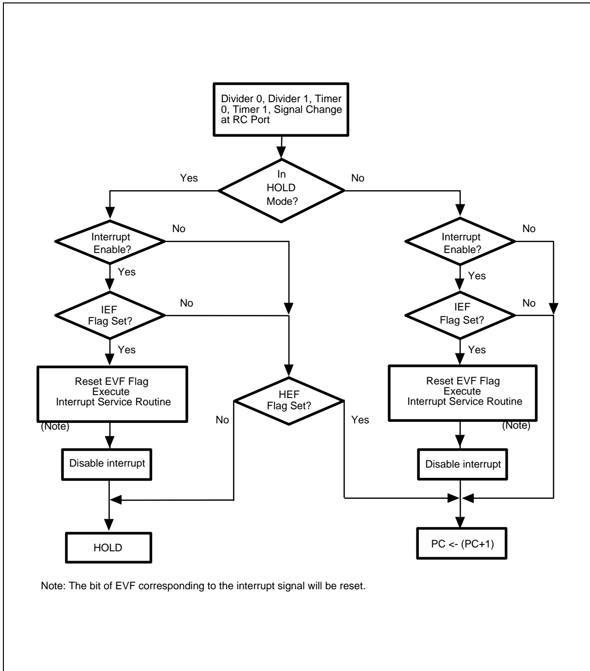
Figure 6-9 Hold Mode and Interrupt Operation Flow Chart
