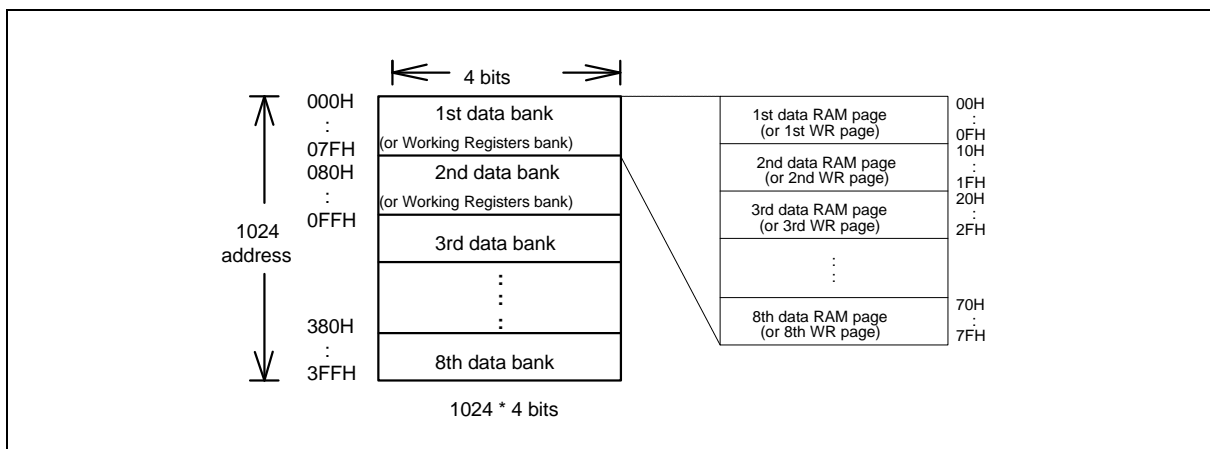
Figure 6-2 Data Memory Organization
