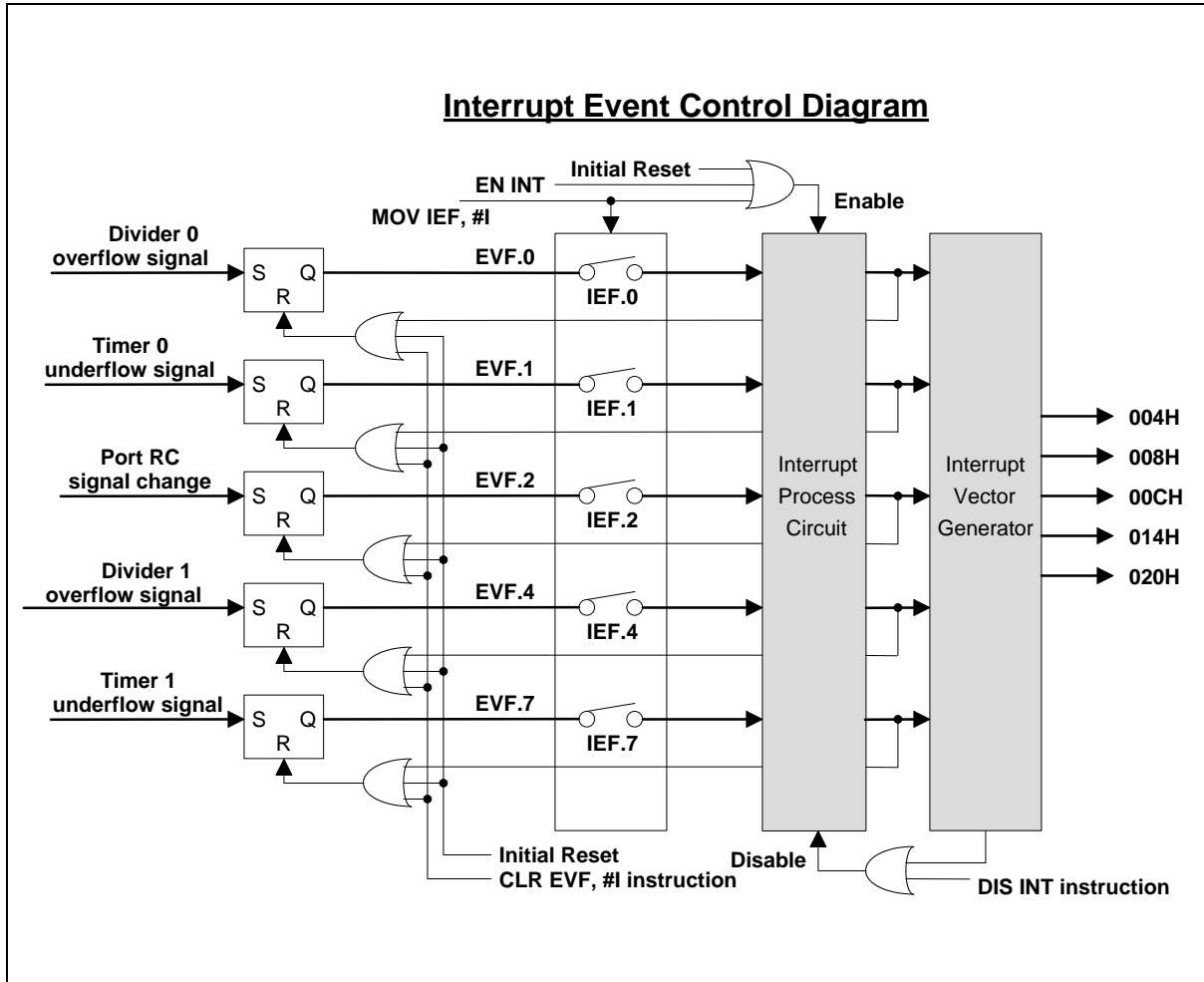
Figure 6-8 Interrupt event control diagram
