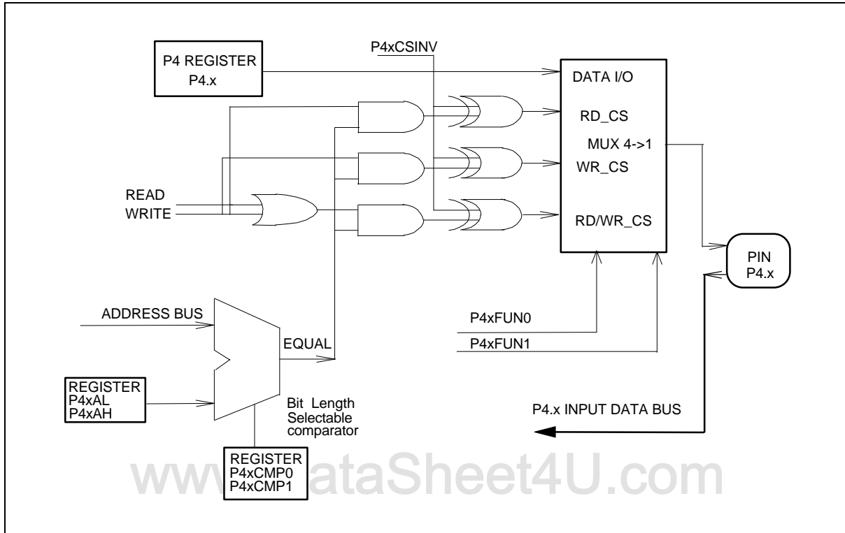
Port 4 Block Diagram
