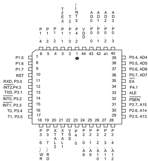
44-Pin PLCC (W78E62BP)
