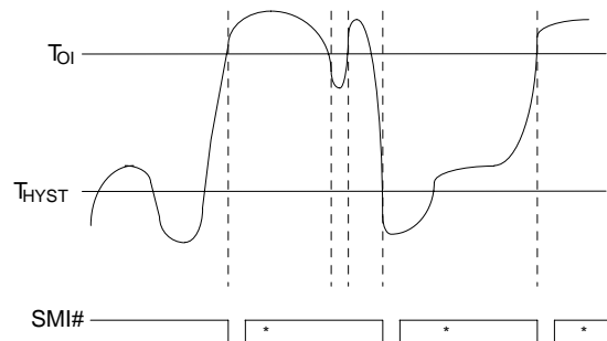
*Interrupt Reset when Interrupt Status Registers are read Figure 6.14
