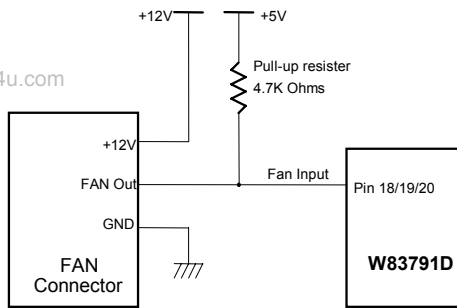
Figure 8-1. Fan with Tach Pull-Up to +5V
