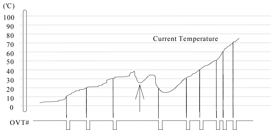
Figure 11-1. ACPI Mode
