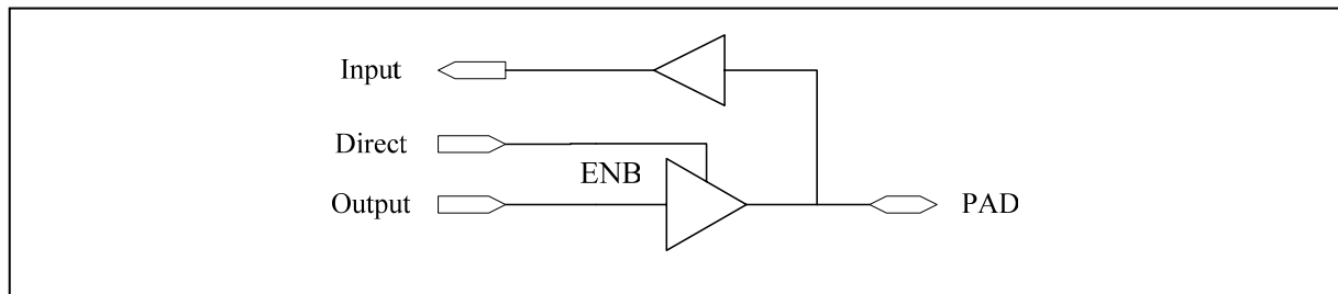
Figure 9-1.GPIO Block Diagram
