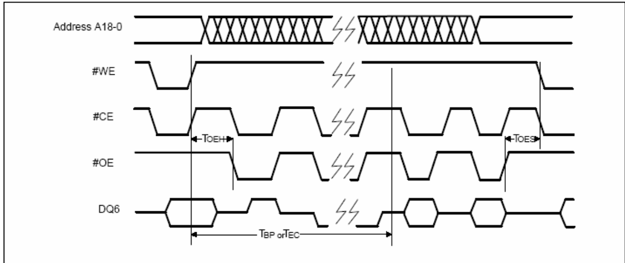
Figure 24-10. Toggle Bit Timing Diagram
