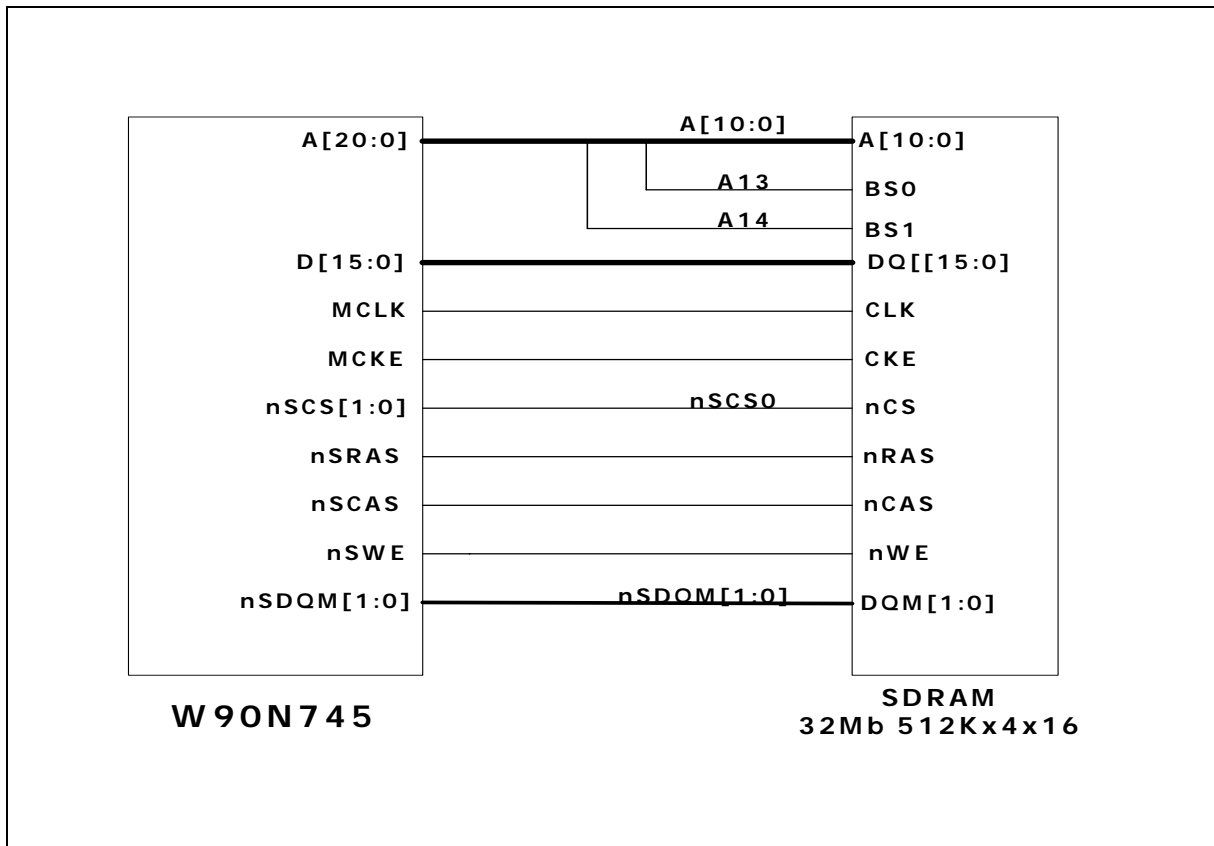
Figure 6.3.1 SDRAM Interface
