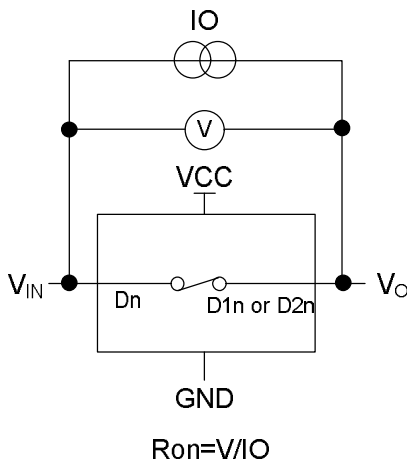
Figure 3: On-Resistance
