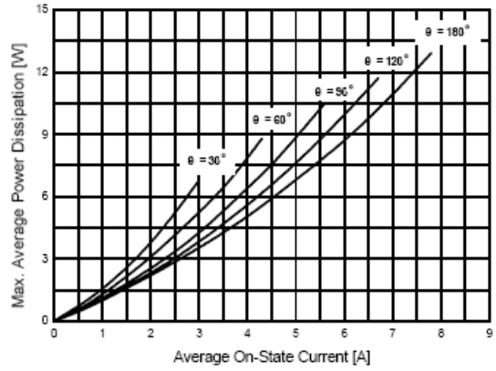
Fig.8 Power Dissipation
