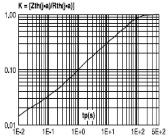
Fig.8 Thermal Resistance junction to ambient Versus copper surface under tab (Epoxy printed Circuit board FR4, copper thickness:35mm)
