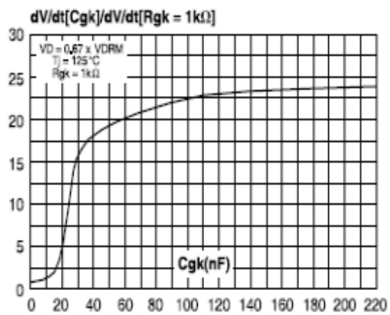
Fig.6 dv/dt VS C_{Gk}
