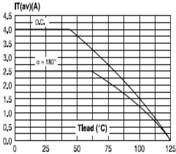
Fig. 1 I_{T(AV)}(DC) vs lead Temperature
