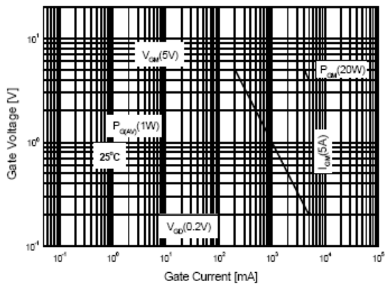
Fig.1 Gate Characteristics
