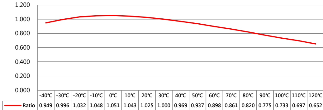
WCS7800 Sensitivity standardization of 30°C (3.3V) V.S Temperature
