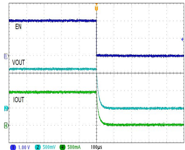
Shutdown from EN
