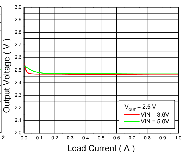
Output voltage vs. Load current
