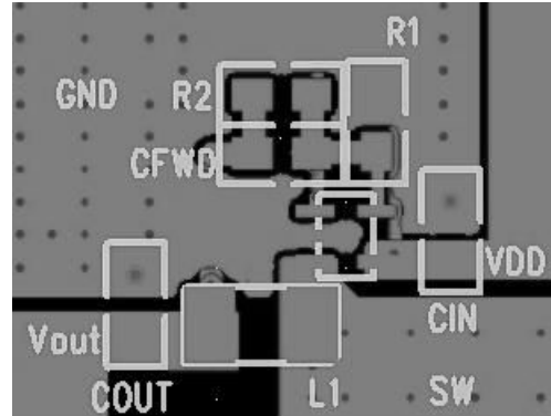
WD1015EA PCB Suggest Layout (Demo)
