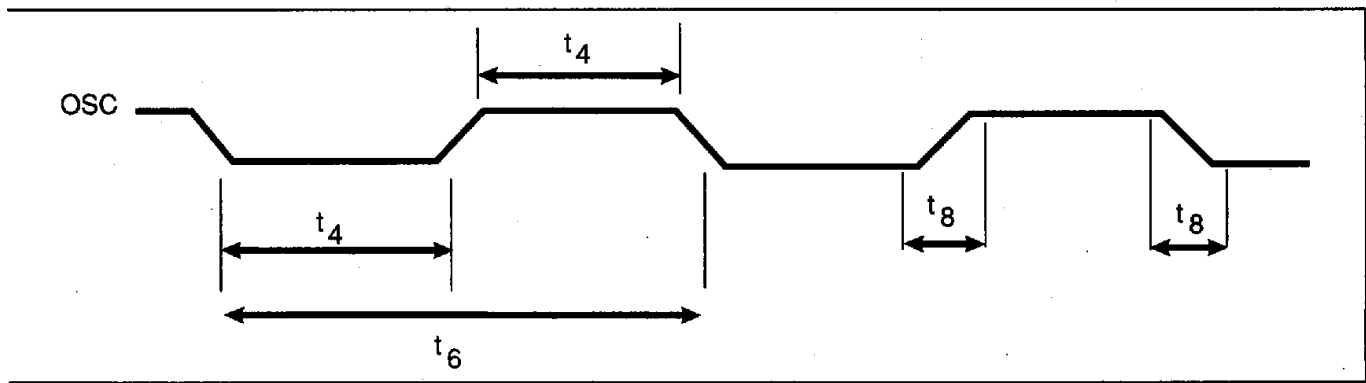
FIGURE 8-2. OSC OUTPUT
