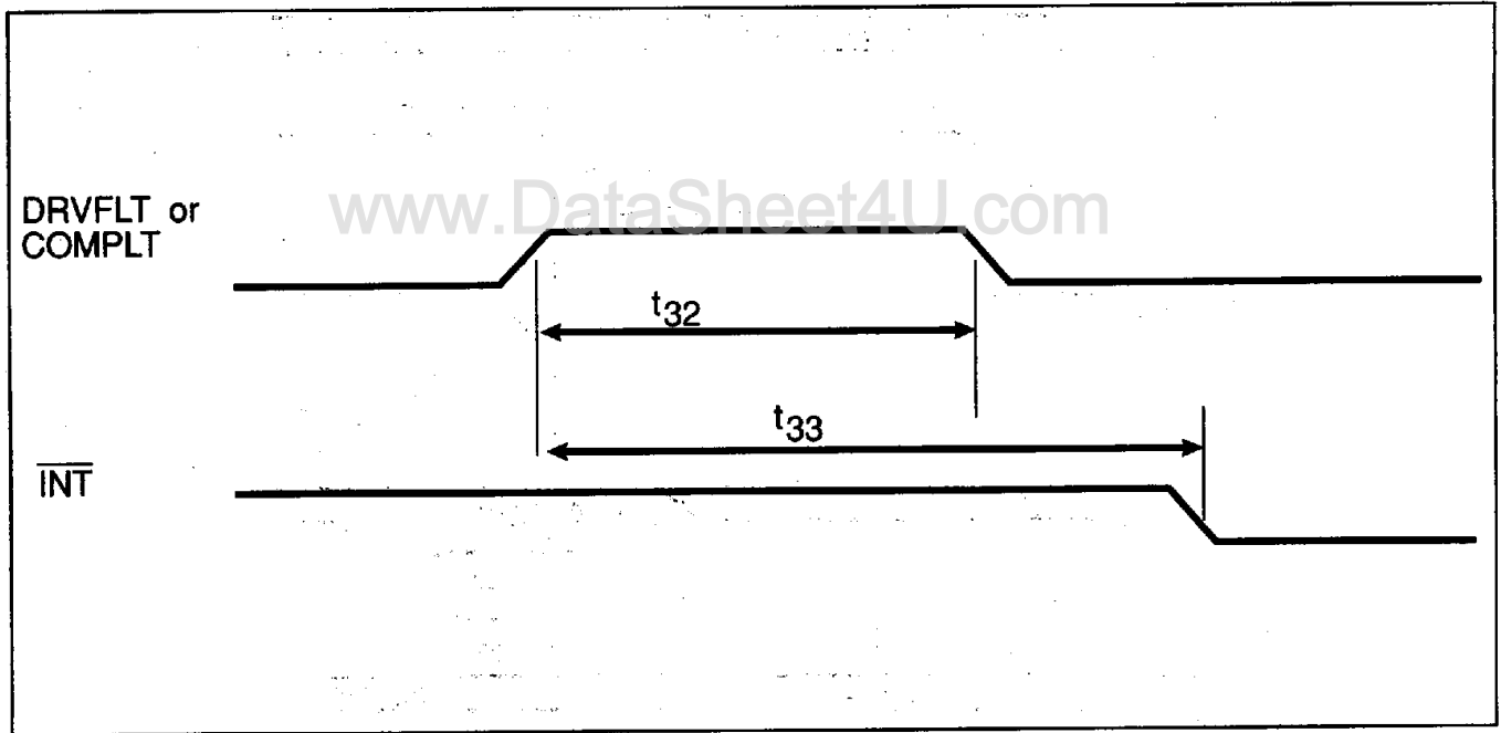
FIGURE 8-9. EXTERNALLY GENERATED INTERRUPT TIMING
