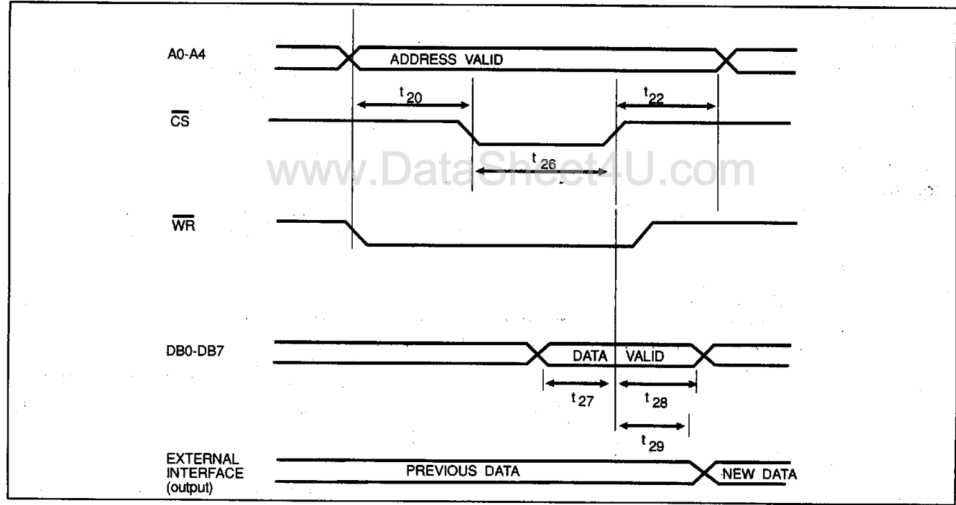
FIGURE 8-7. MICROPROCESSOR WR* TIMING (CS* CONTROLLED)
