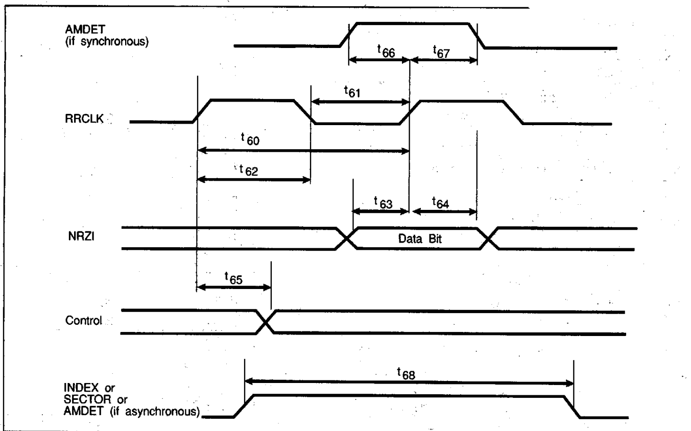
FIGURE 8-14. NRZ DATA INPUT TIMING
