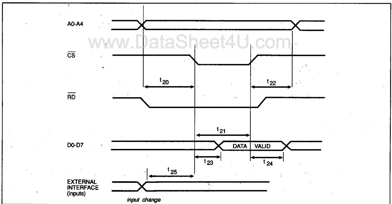
FIGURE 8-5. MICROPROCESSOR RD* TIMING (CS* CONTROLLED)
