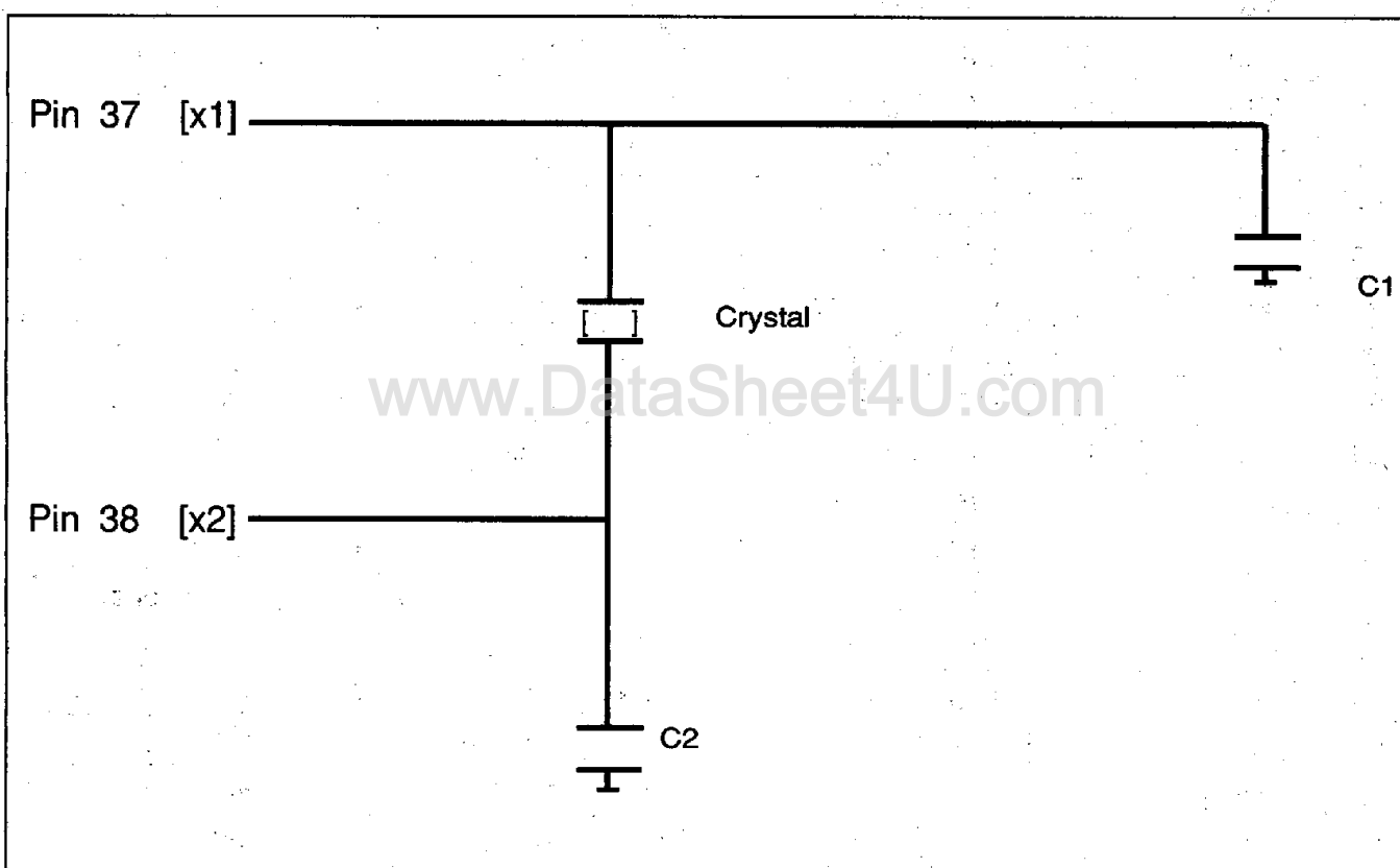
FIGURE C-1. OSCILLATOR WITH CAPACITORS
