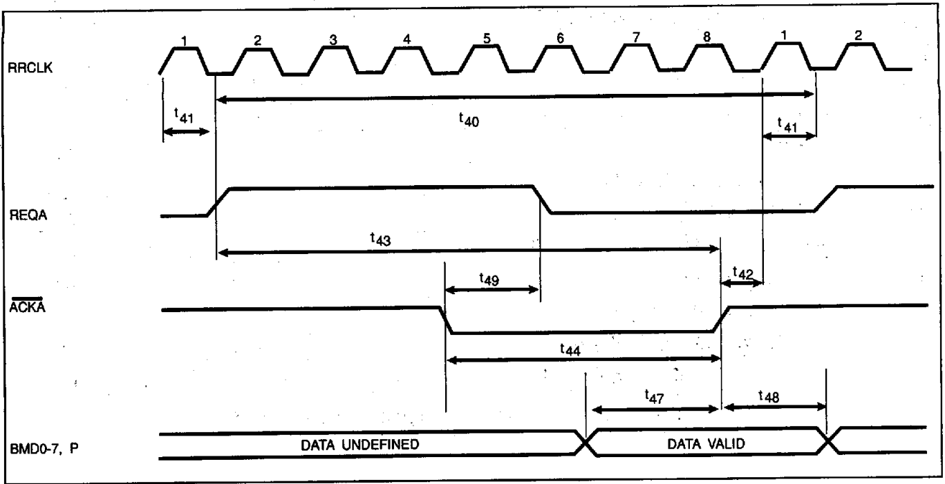
FIGURE 8-10. ASYNCHRONOUS MODE DATA BUS WRITE TIMING (1)
