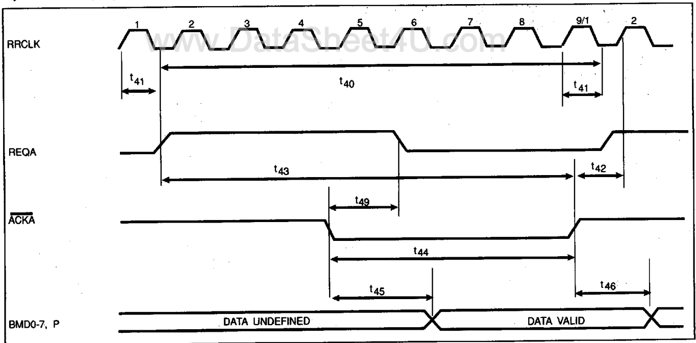
FIGURE 8-11. ASYNCHRONOUS MODE DATA BUS READ TIMING (0)
