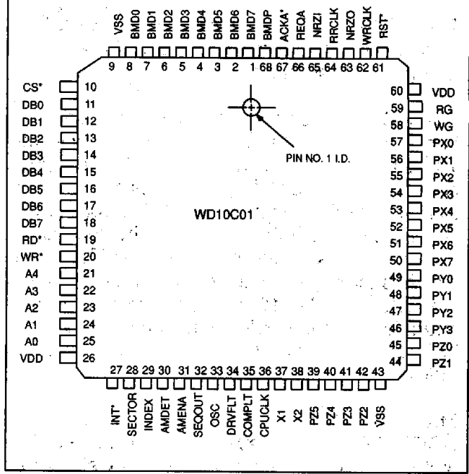
FIGURE 1-1. 68-PIN PLCC
