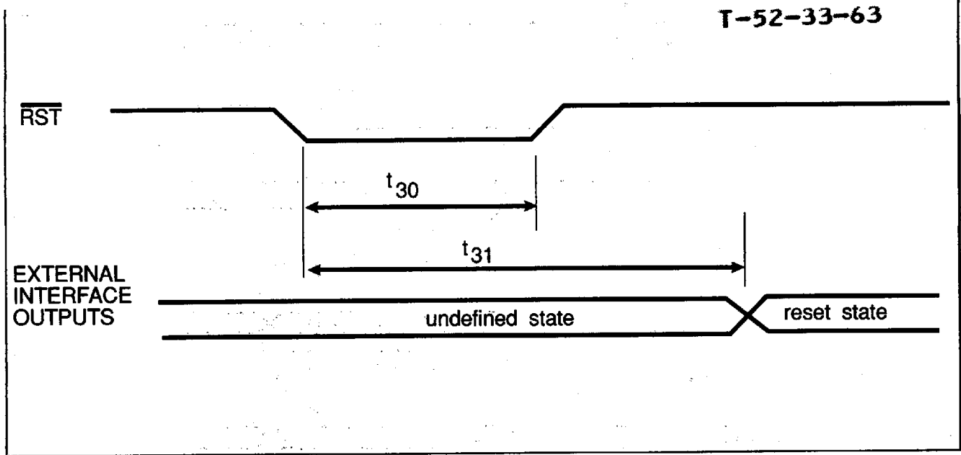
FIGURE 8-8. RESET TIMING
