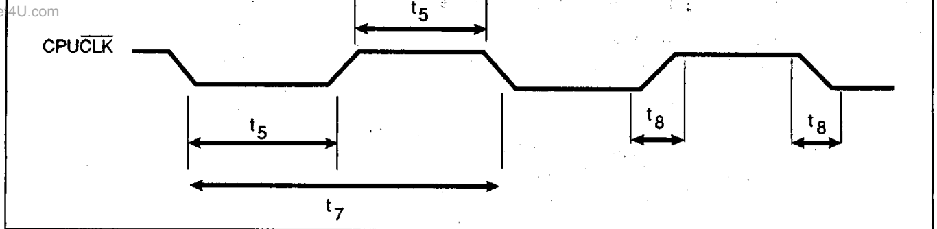
FIGURE 8-3. CPUCLK OUTPUT
