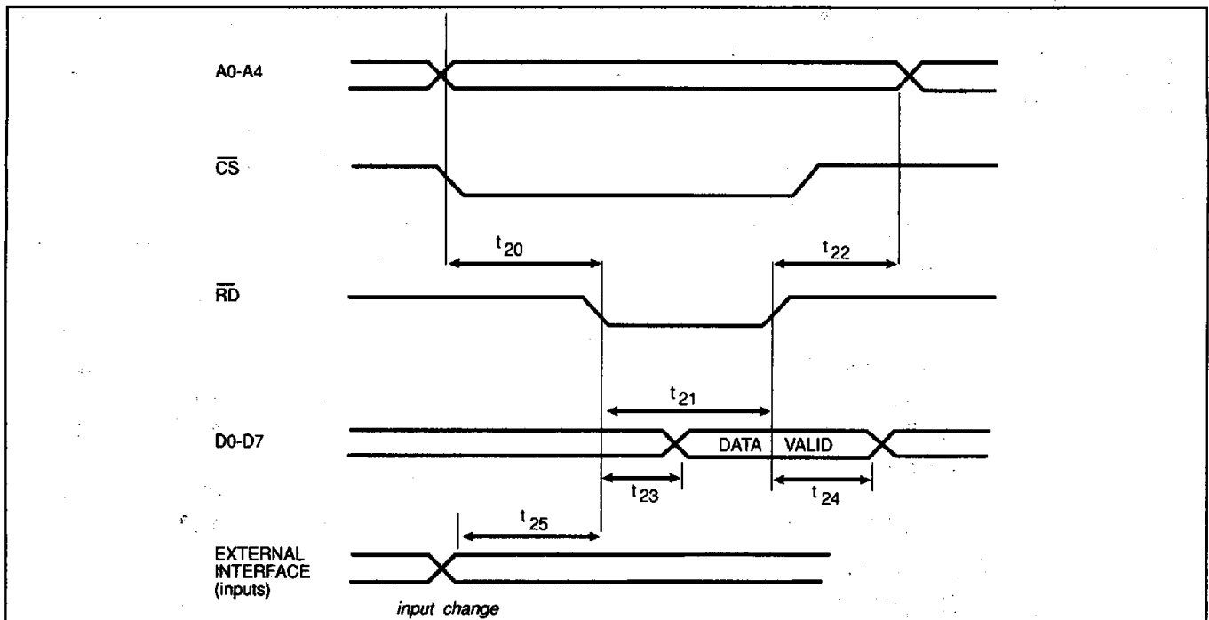
FIGURE 8-4. MICROPROCESSOR RD* TIMING (RD* CONTROLLED)
