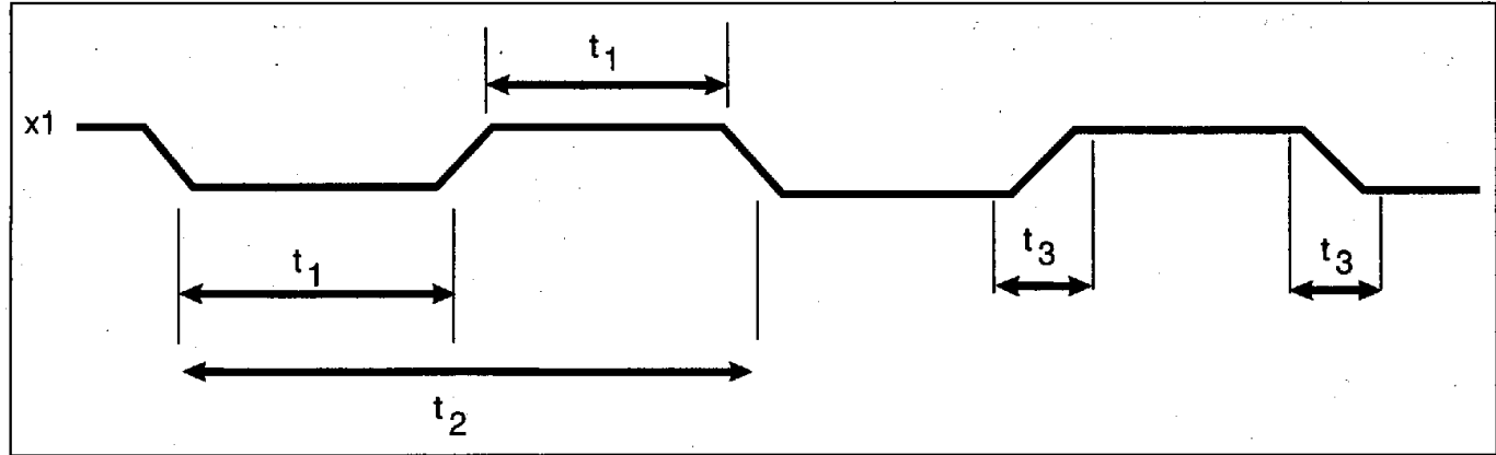
FIGURE 8-1. TTL SOURCE X1 CLOCK INPUT
