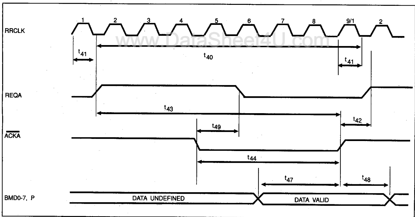
FIGURE 8-13. ASYNCHRONOUS MODE DATA BUS WRITE TIMING (0)
