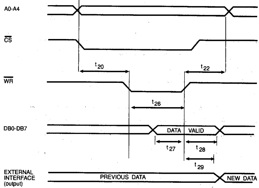
FIGURE 8-6. MICROPROCESSOR WR* TIMING (WR* CONTROLLED)
