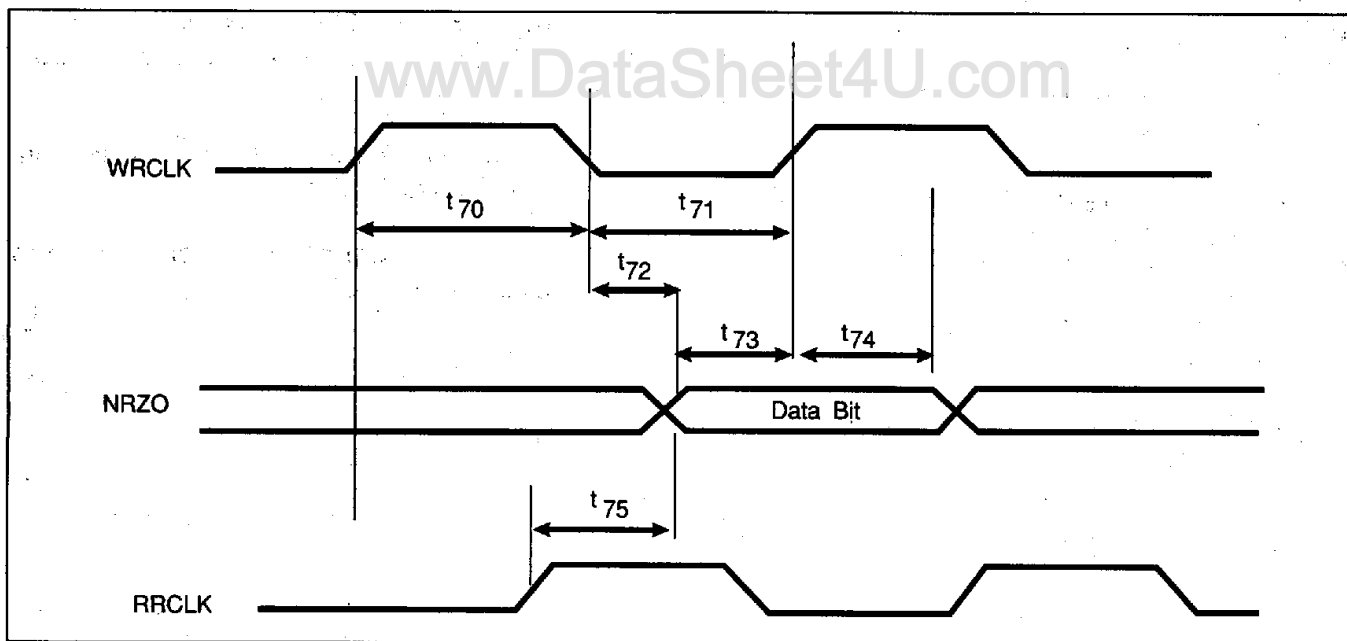
FIGURE 8-15. NRZ DATA OUTPUT TIMING
