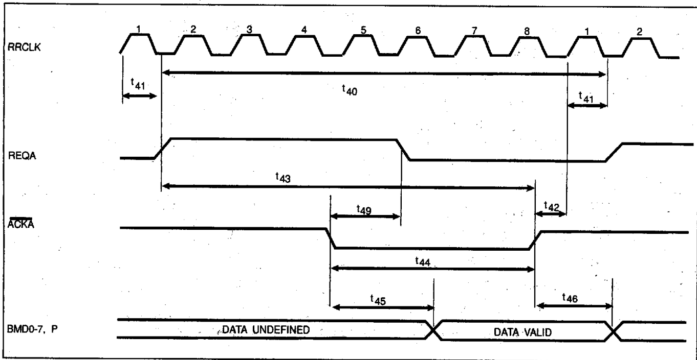
FIGURE 8-12. ASYNCHRONOUS MODE DATA BUS READ TIMING (1)
