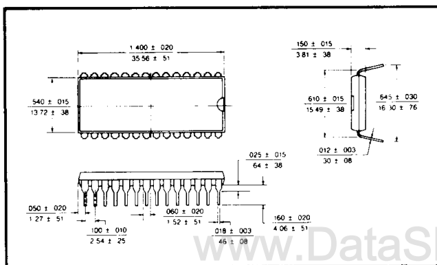
28 LEAD PLASTIC PH
