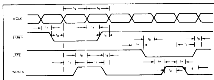
FIGURE 4. WRITE SETUP/OLD
