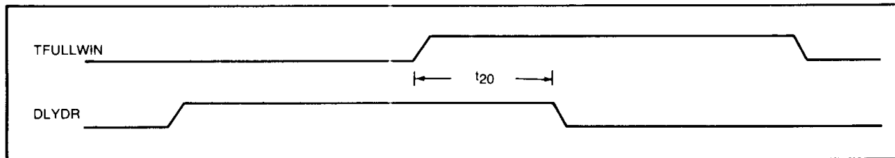
FIGURE 7. DLYDR, TFULLWIN TIMING
