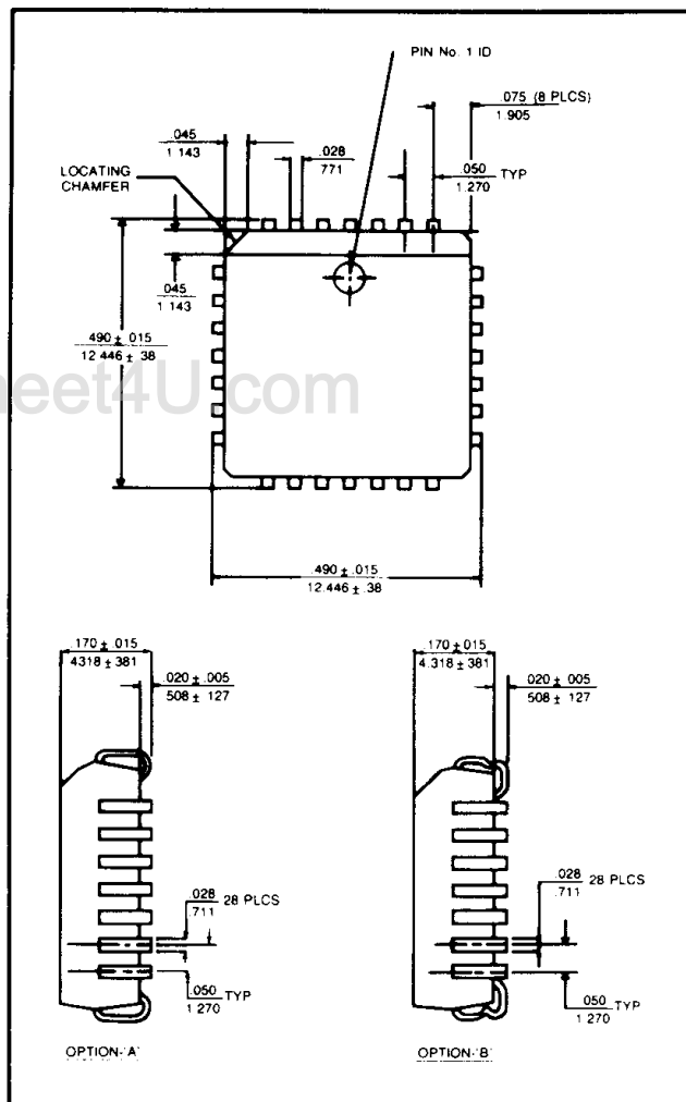
28 LEAD PLASTIC QUAD JH
