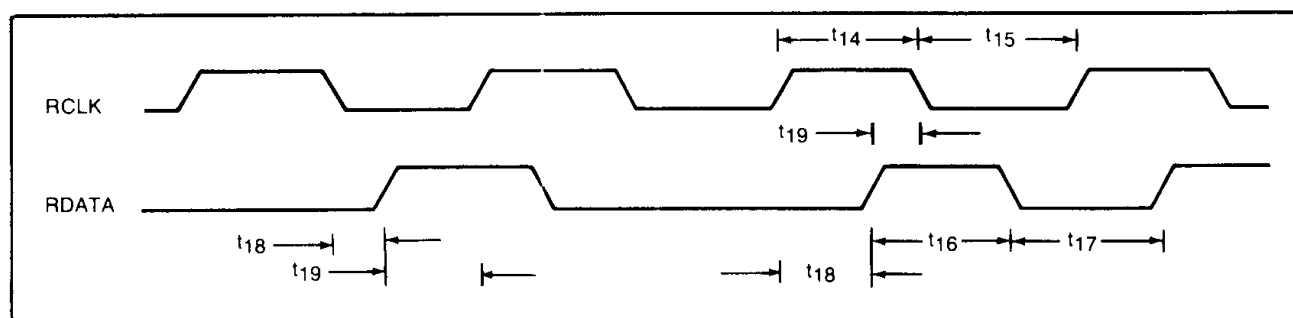
FIGURE 6. RCLK, RDATA TIMING
