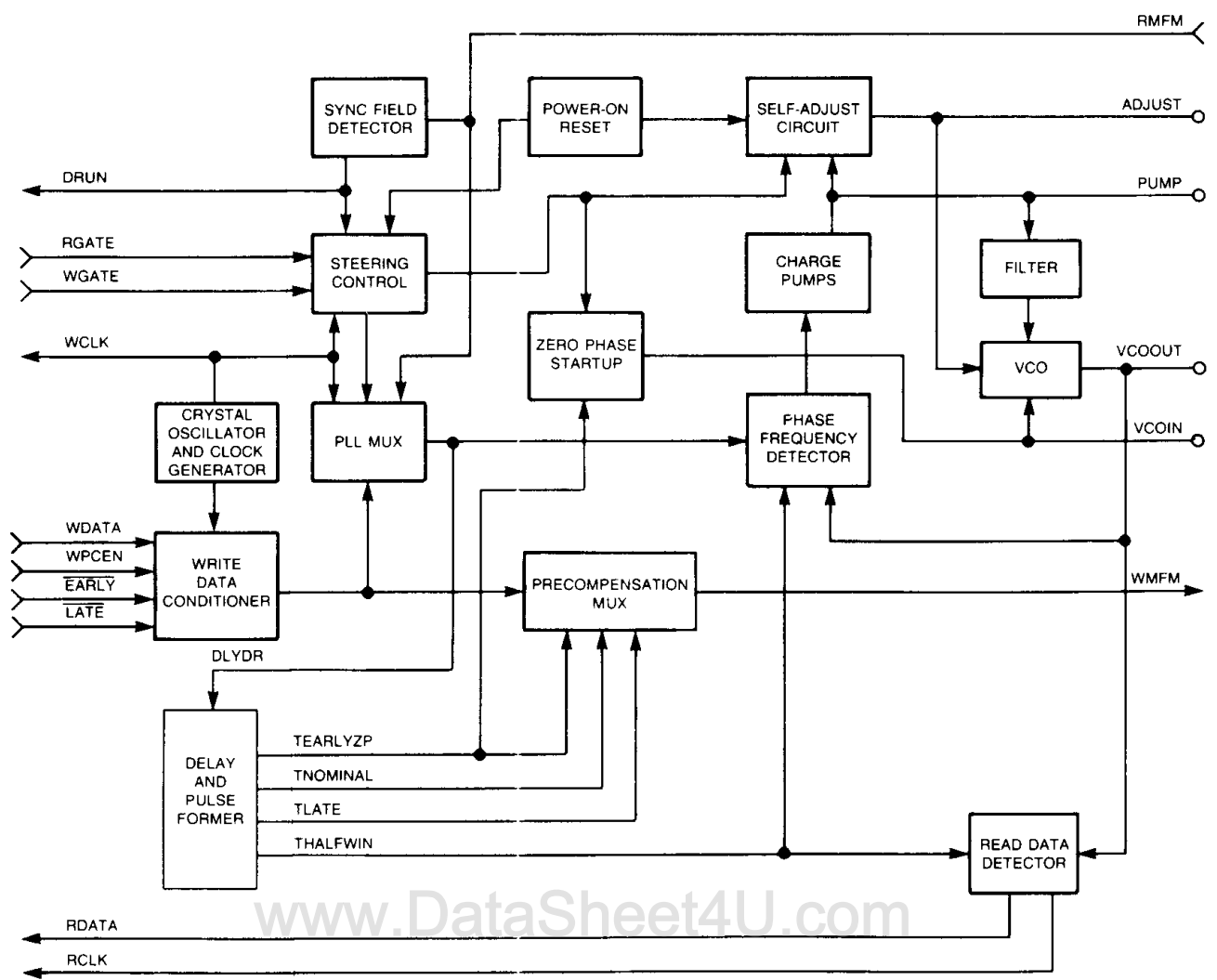
FIGURE 2. WD10C20 BLOCK DIAGRAM
