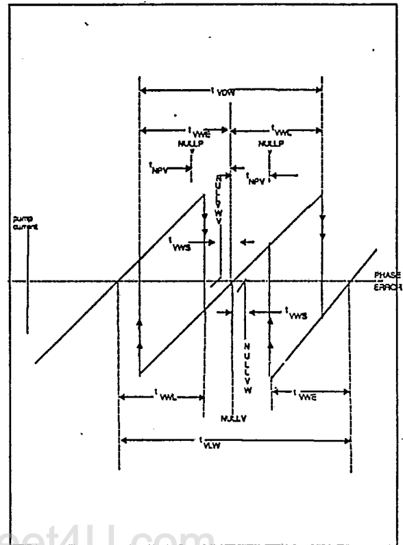
FIGURE 9. VELOCITY LOCK MODE
