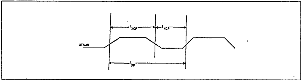
FIGURE 11. TTL XTALIN INPUT CLOCK
