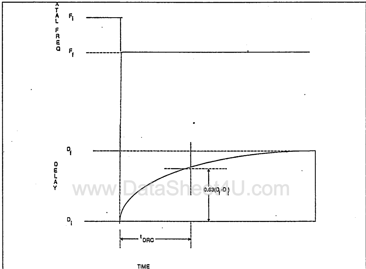
TIME FIGURE 13. DELAY LINE TIMING
