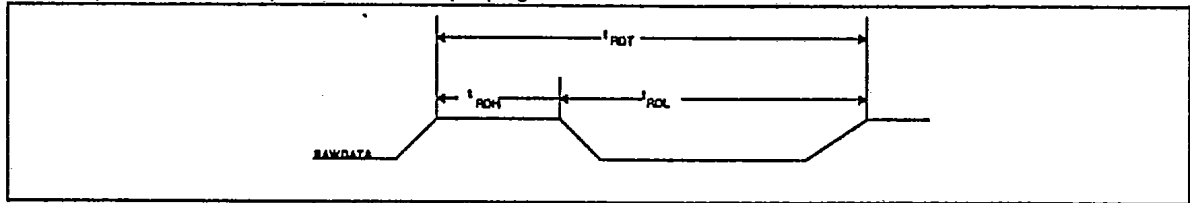
Figure 5. DISK DRIVE READ DATA TIMING
