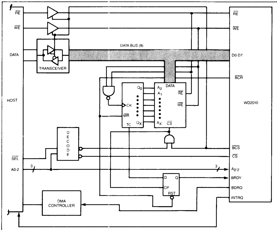
FIGURE 2. HOST INTERFACE
