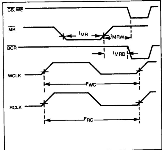
MISCELLANEOUS TIMING
