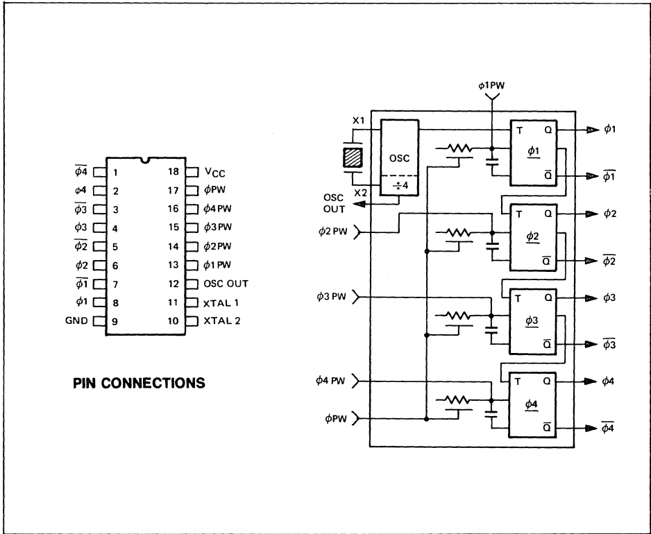
WD2143-01 BLOCK DIAGRAM
