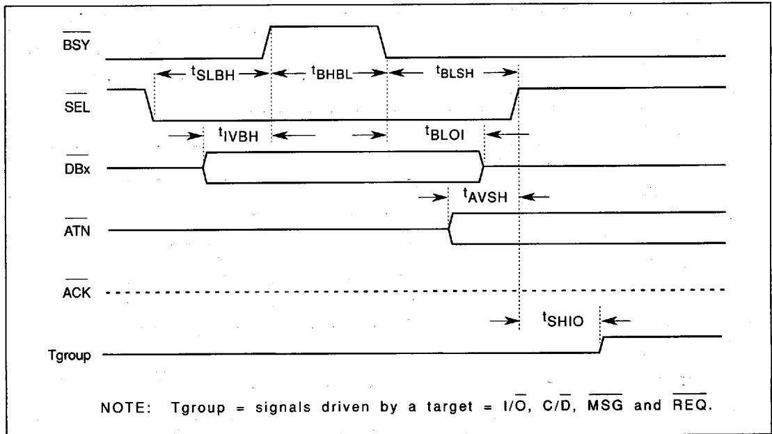
FIGURE 6-16. TIMING-TARGET RESPONSE
