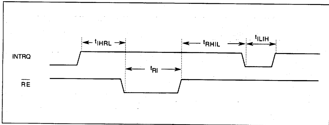
FIGURE 6-13. INTRQ TIMING
