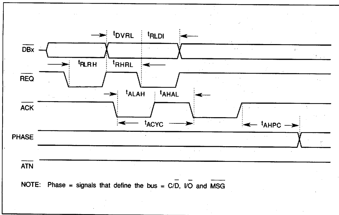
FIGURE 6-25. TIMING-SEND SYNCHRONOUS TRANSFER IN AS TARGET
