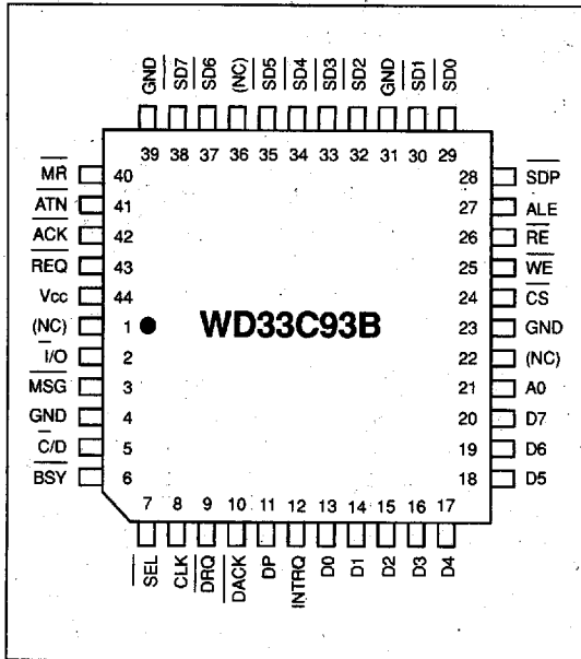
FIGURE 2-1. 44-PIN PLCC
