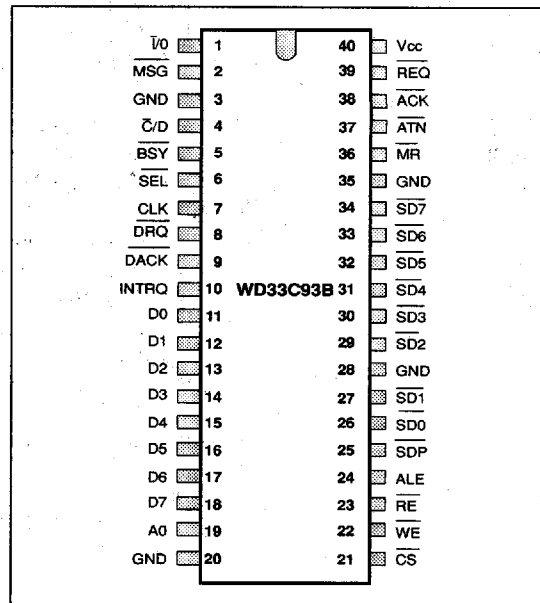
FIGURE 2-2. 40-PIN DIP
