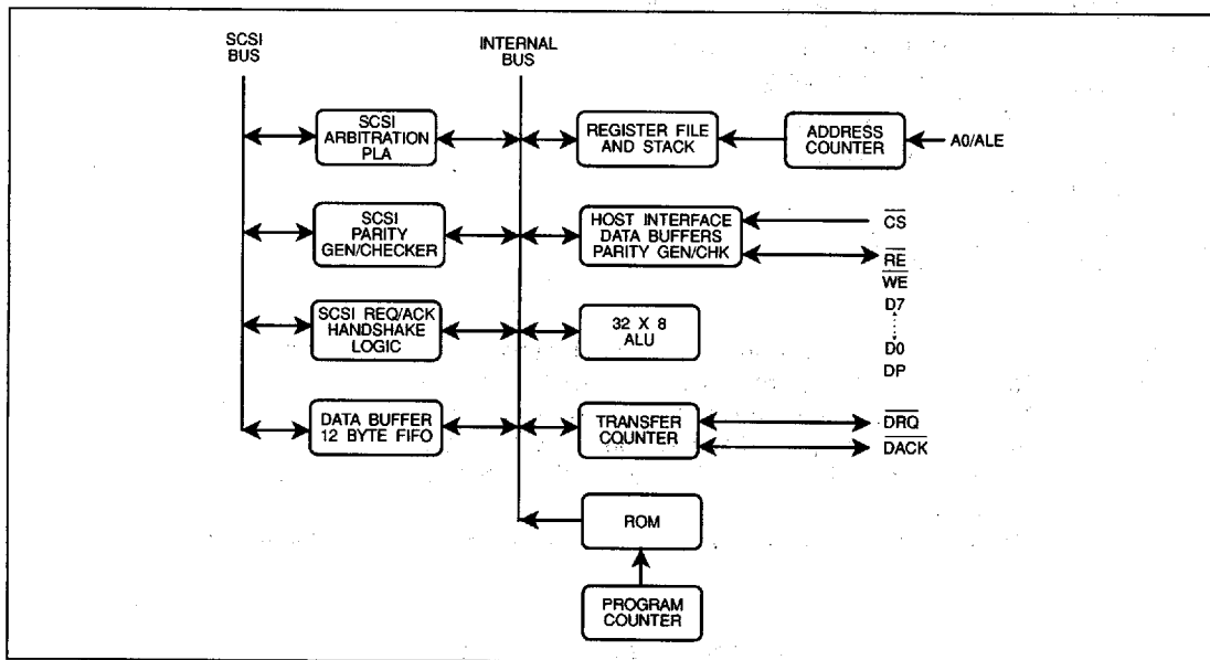
FIGURE 2-3. WD33C93B BLOCK DIAGRAM
