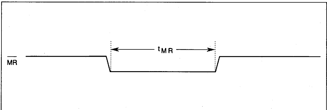
FIGURE 6-2. \overline{MR} -TIMING
