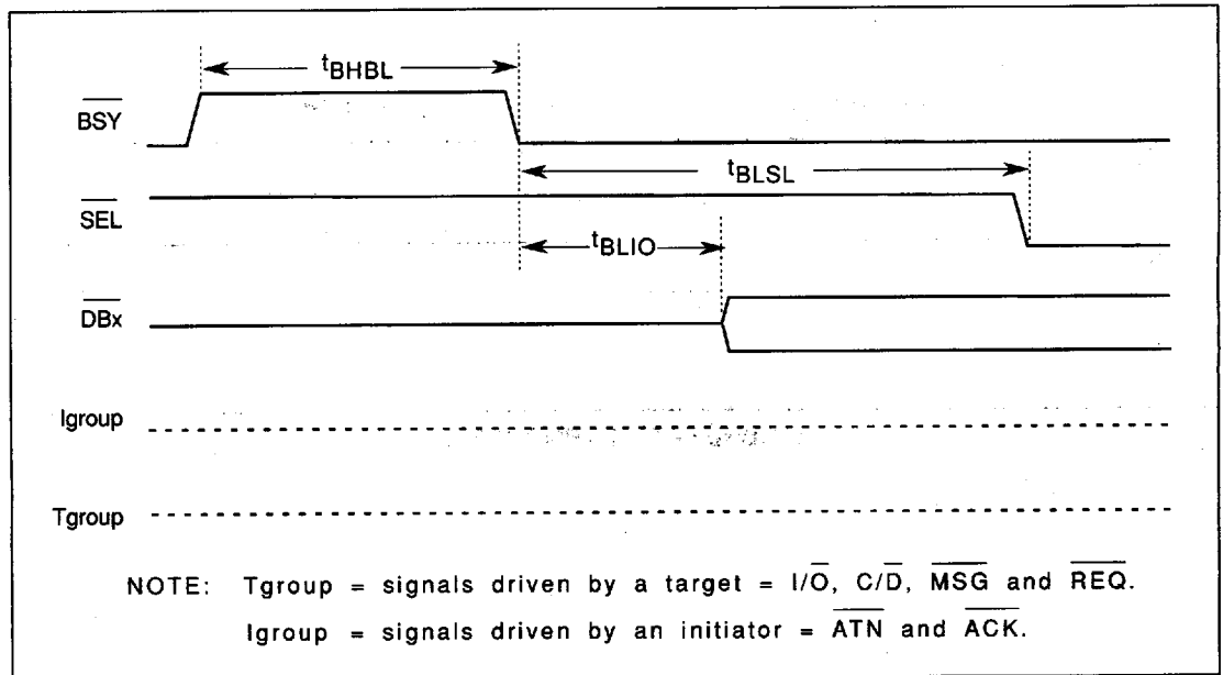
FIGURE 6-14. ARBITRATION TIMING
