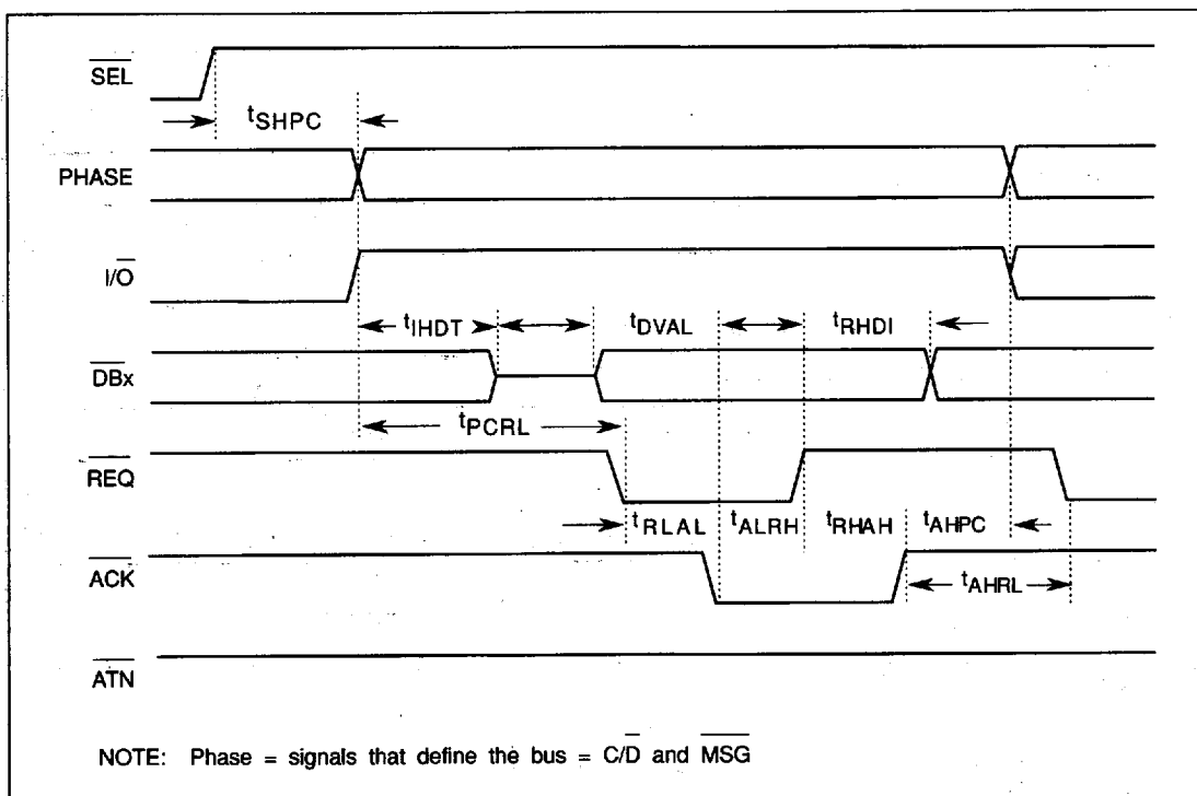
FIG. 6-22. TIMING-RECEIVE ASYNCHRONOUS TRANSFER OUT AS TARGET
