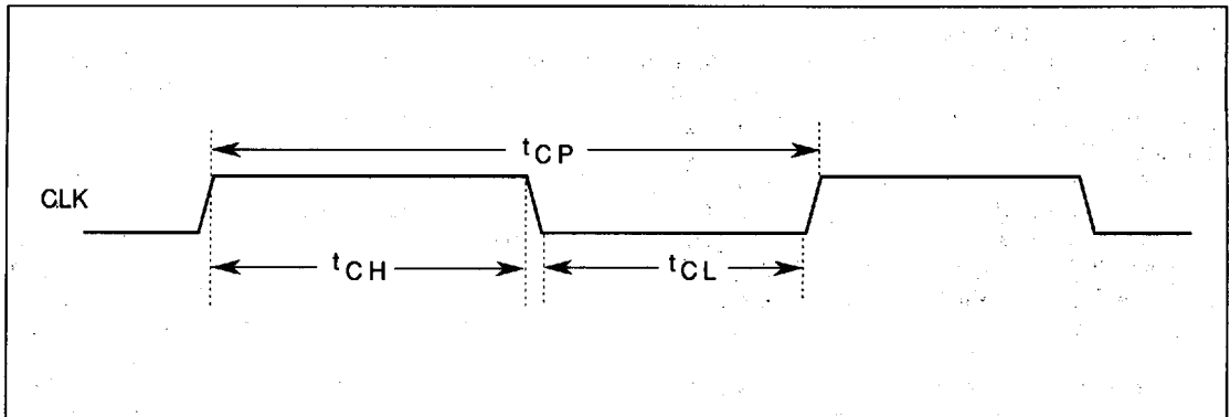
FIGURE 6-1. CLOCK TIMING
