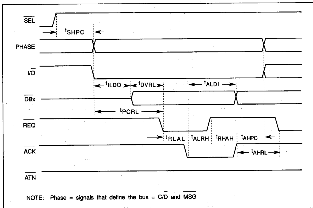
FIGURE 6-20. TIMING-ASYNCHRONOUS TRANSFER IN AS TARGET
