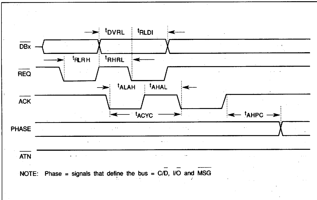
FIGURE 6-24. TIMING-SEND SYNCHRONOUS TRANSFER IN AS TARGET
