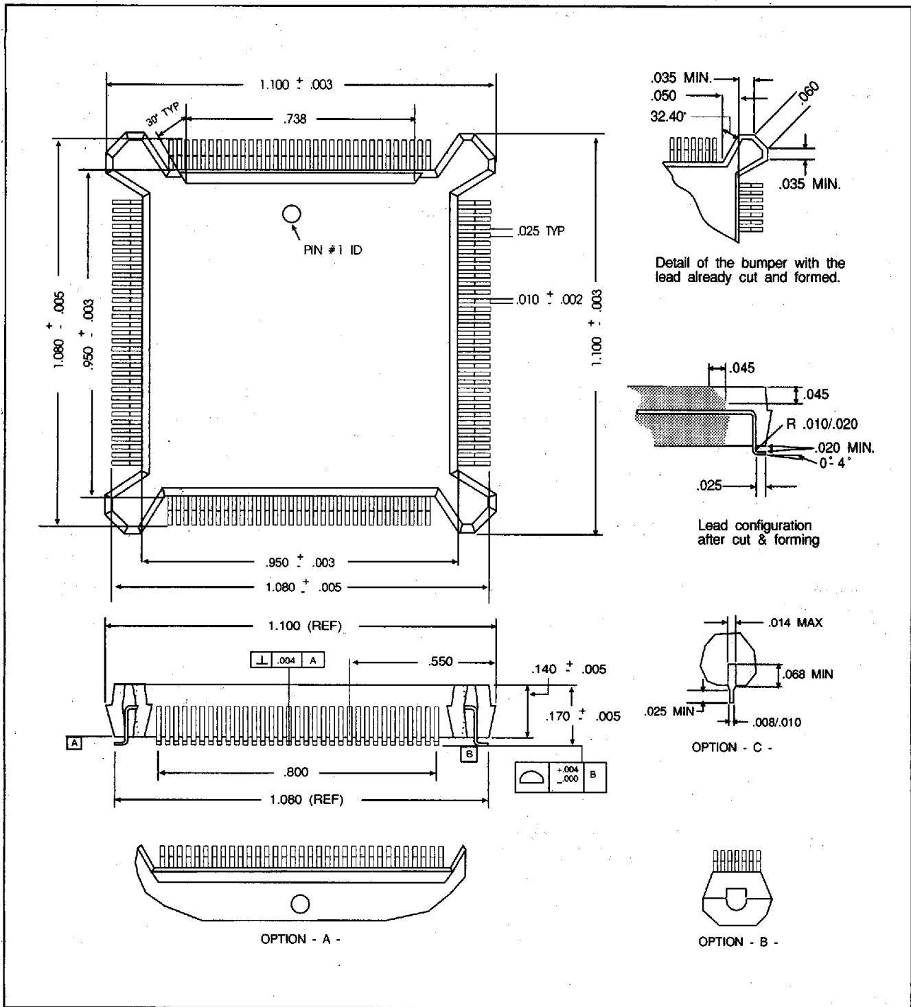
FIGURE 20-1. 132-PIN PQFP PACKAGE
