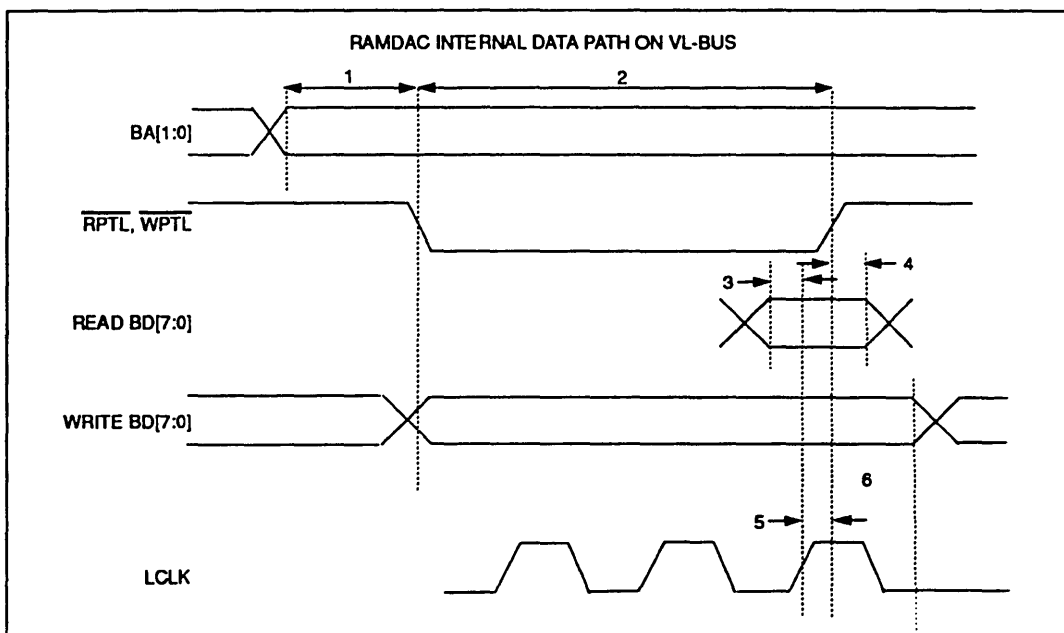
FIGURE 19-5. RAMDAC TIMING
