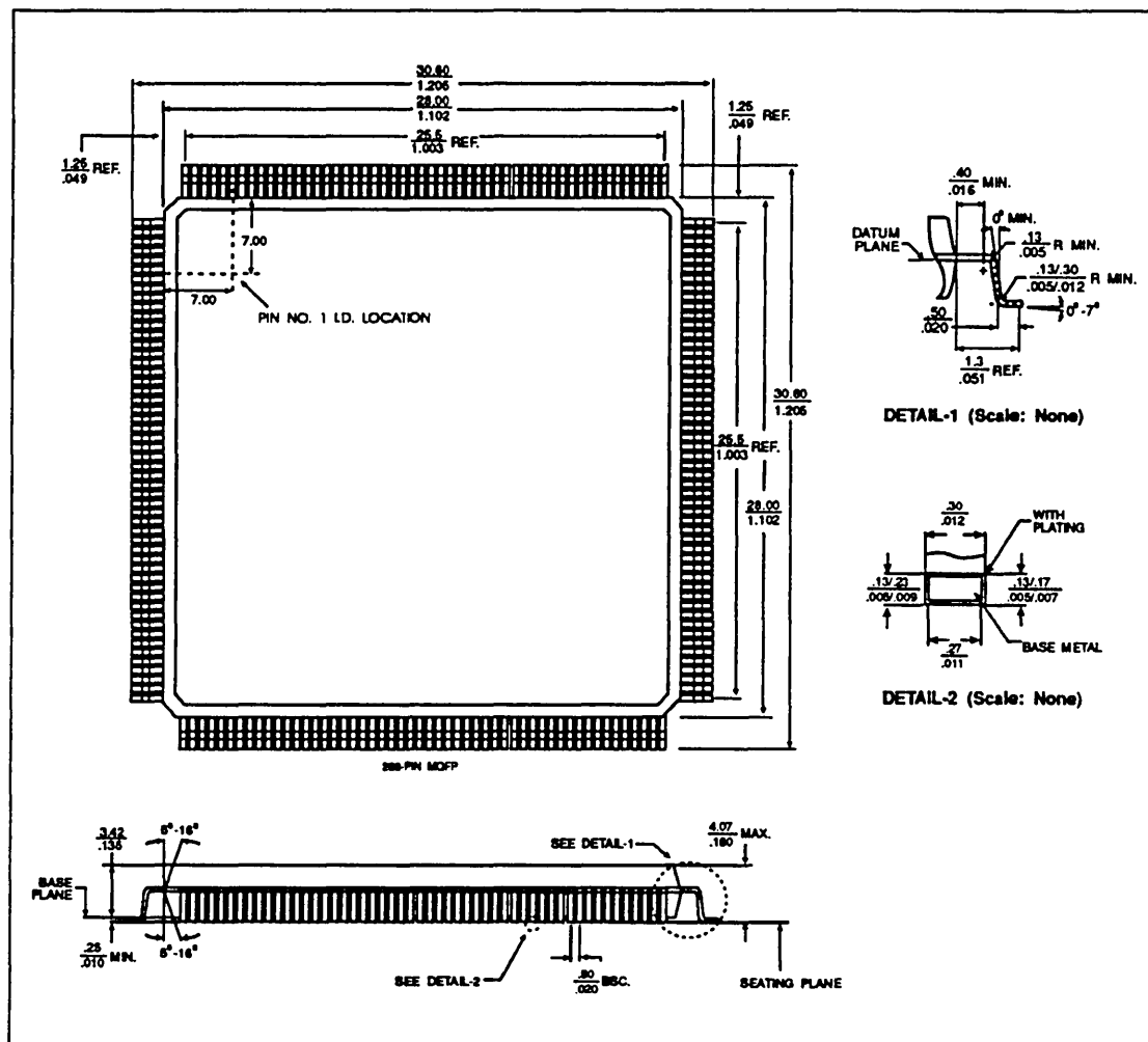
FIGURE 20-1. 208-PIN MQFP PACKAGE DIMENSIONS
