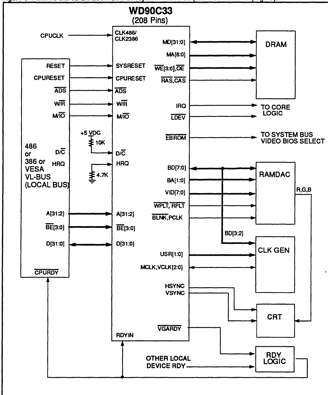
FIGURE 3-3. LOCAL BUS SUBSYSTEM INTERFACE, 32-BIT
