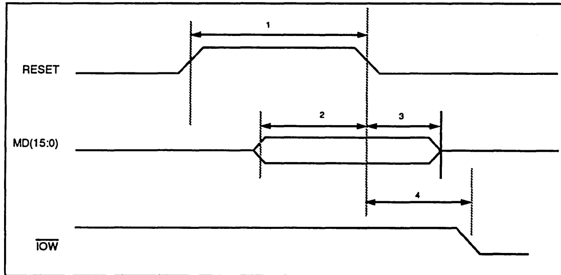
FIGURE 19-1. RESET TIMING
