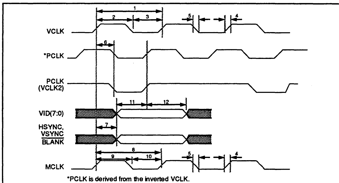
FIGURE 19-2. CLOCK AND VIDEO TIMING
