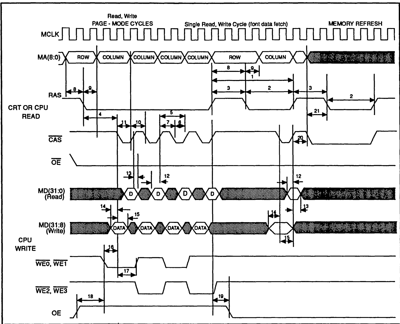
FIGURE 19-6. DRAM TIMING
