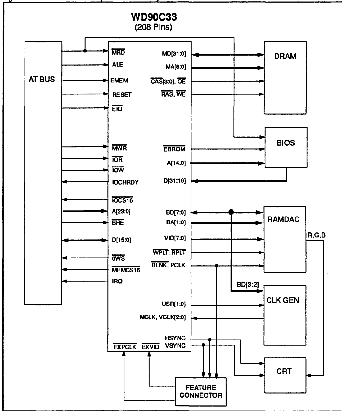
FIGURE 3-4. AT COMPATIBLE BUS SUBSYSTEM
