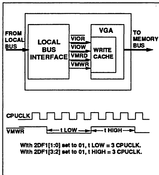
FIGURE 10-1 LOCAL BUS INTERNAL COMMAND WIDTH ADJUSTMENT
