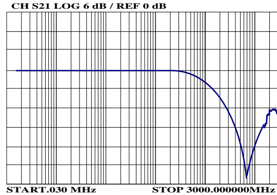
Figure 2: Insertion Loss
