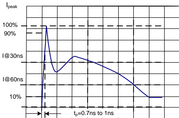
Figure 4. IEC 61000-4-2 Waveform
