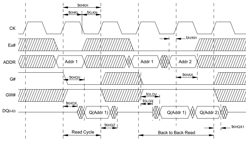
SYNCHRONOUS ONLY READ CYCLE
