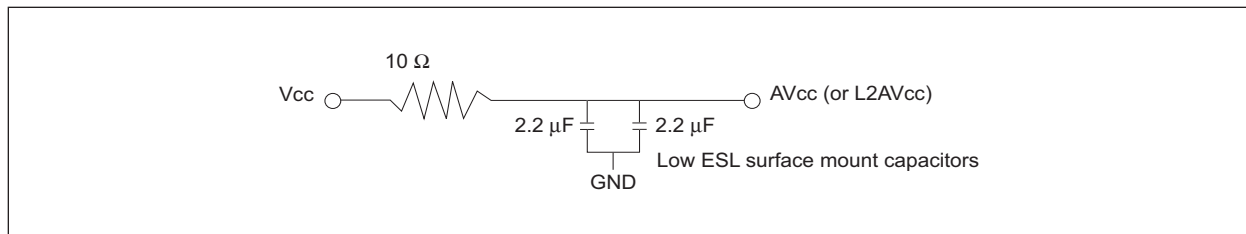
FIGURE 6 – POWER SUPPLY FILTER CIRCUIT
