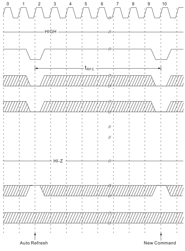
FIG. 18 AUTO REFRESH CYCLE
