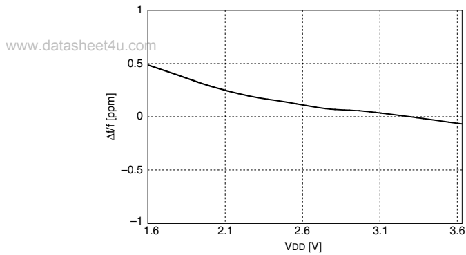
5027×D, f_{OUT} = 85\text{MHz} , 3.3V standard, T_a = 25^\circ\text{C}
