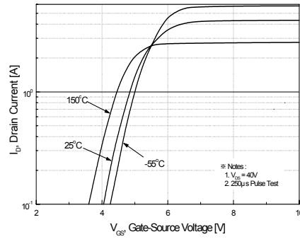
Figure 2. Transfer Characteristics
