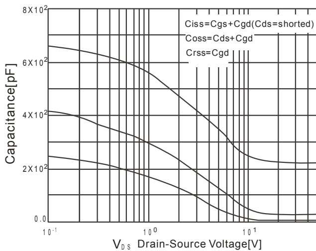
Fig.5 Capacitance Characteristics
